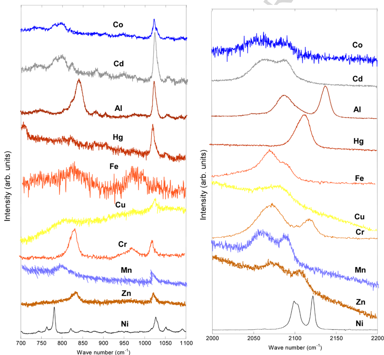
Figure 5. Raman spectra of the ten metal thiocyanate ILs between 700 and 1100, and 2000 and 2200 \text{cm}^{-1} at 300 K where the [\text{M}(\text{SCN})]^- ( \text{M} = \text{Metal} ) bands are presented.
