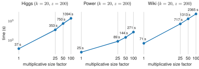
Figure 5: Scalability with respect to input size of the randomized MapReduce algorithm for the k -center problem with z outliers, using coresets of size 8 \cdot (k + 6 \cdot z/\ell) and parallelism 16. Both axes are in logarithmic scale.
