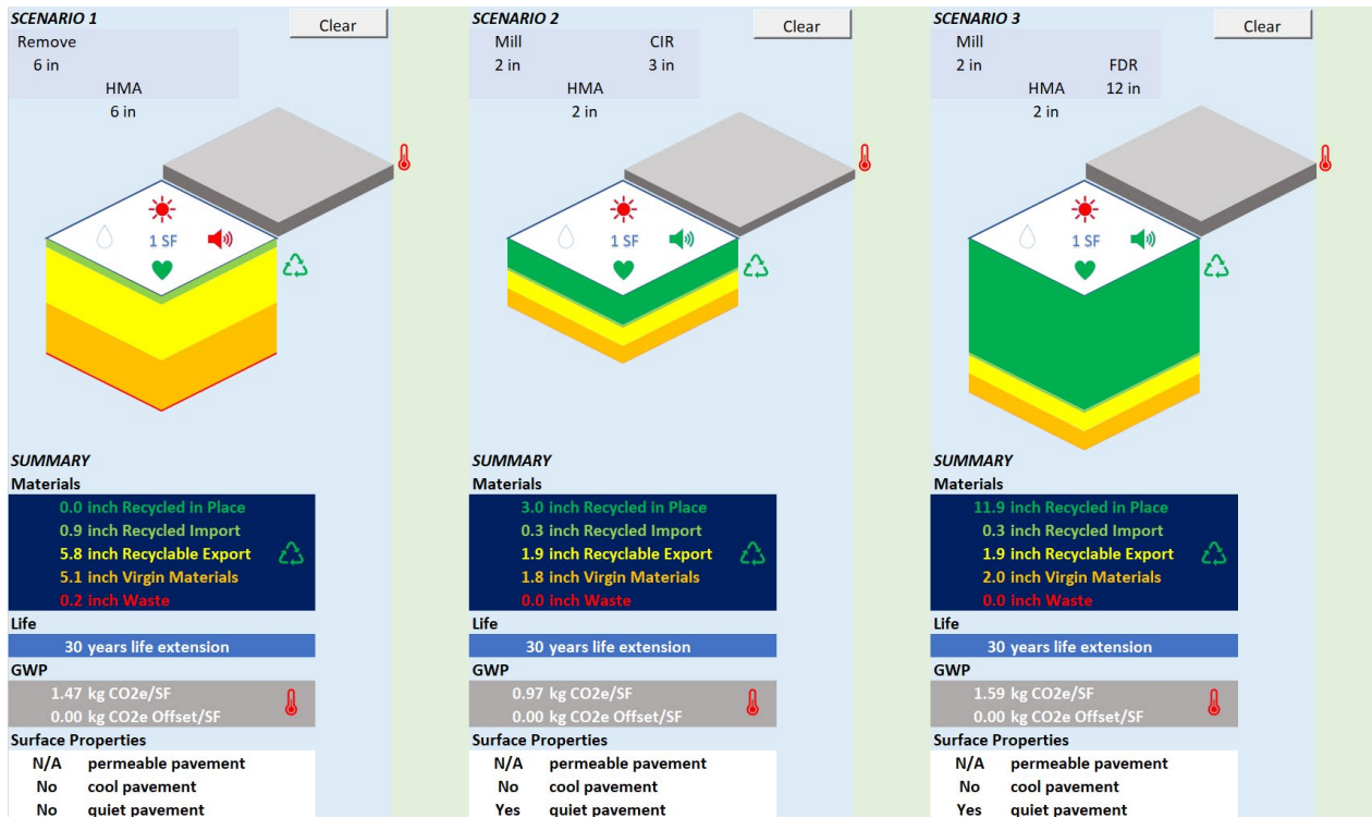
Figure 13. Flexible Pavement Rehabilitation Example.
