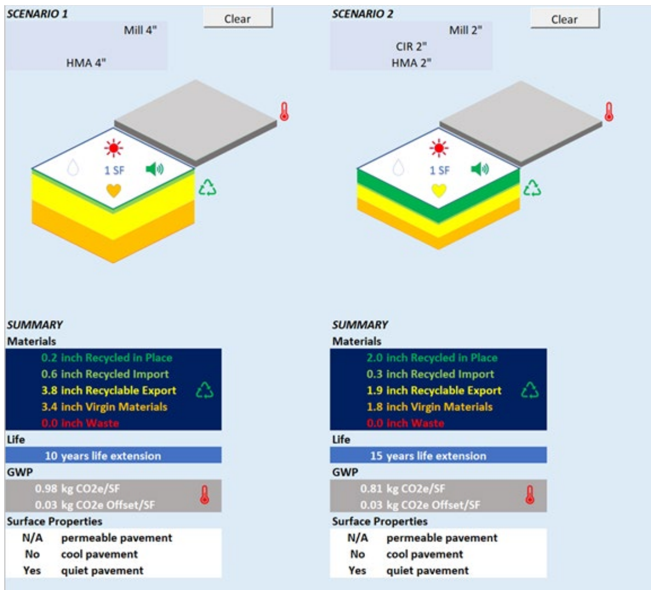
Figure 1. Comparison of Pavement Rehabilitation Scenarios Using Green Up
