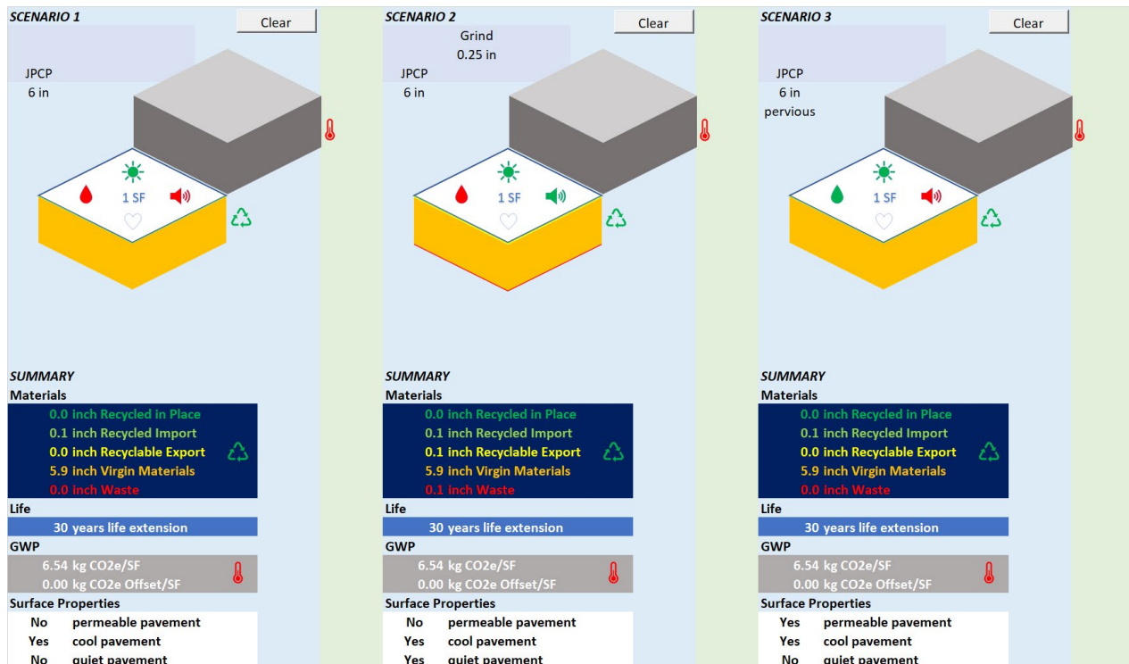
Figure 7. Green Up Graphic for 6 in. JPCP, JPCP + Diamond Grinding, and Pervious Concrete
