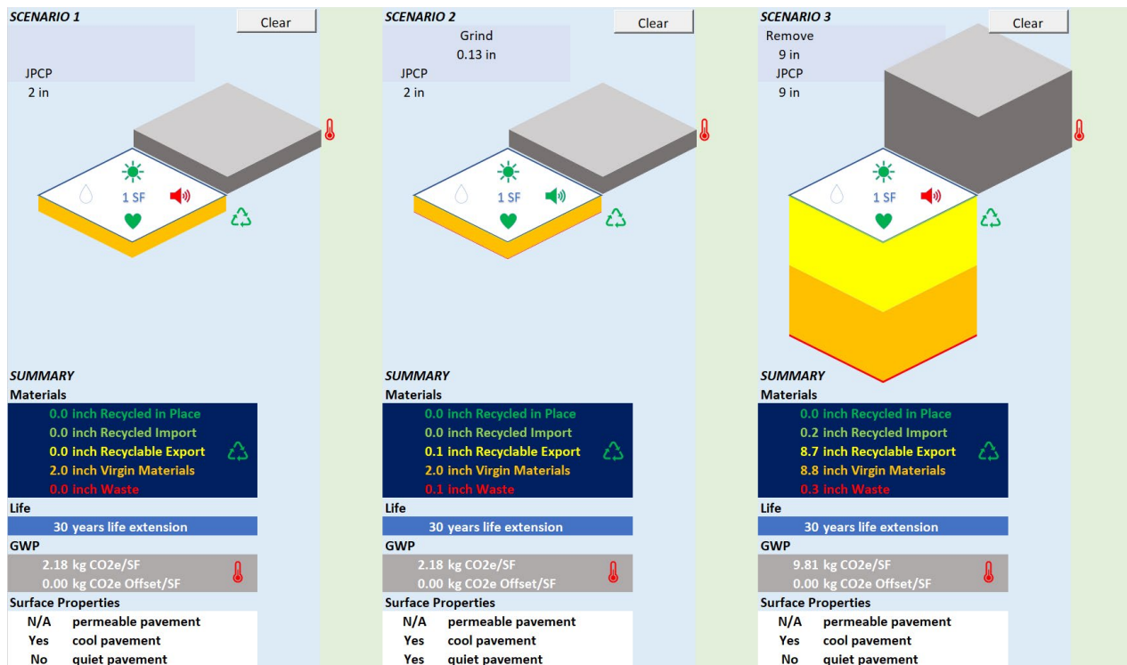
Figure 12. Rigid Pavement Rehabilitation Example
