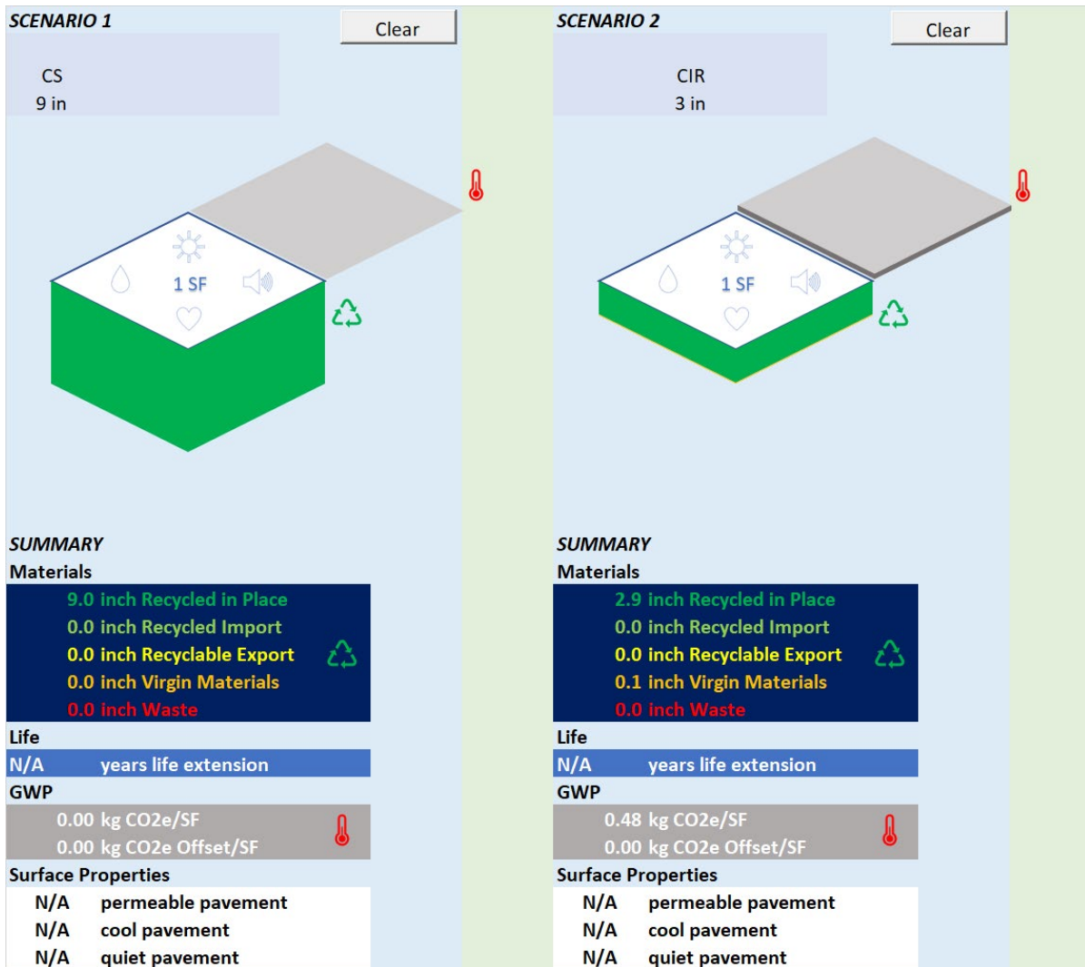
Figure 5. Green Up Graphic for 9 in. CS, 3 in. CIR
