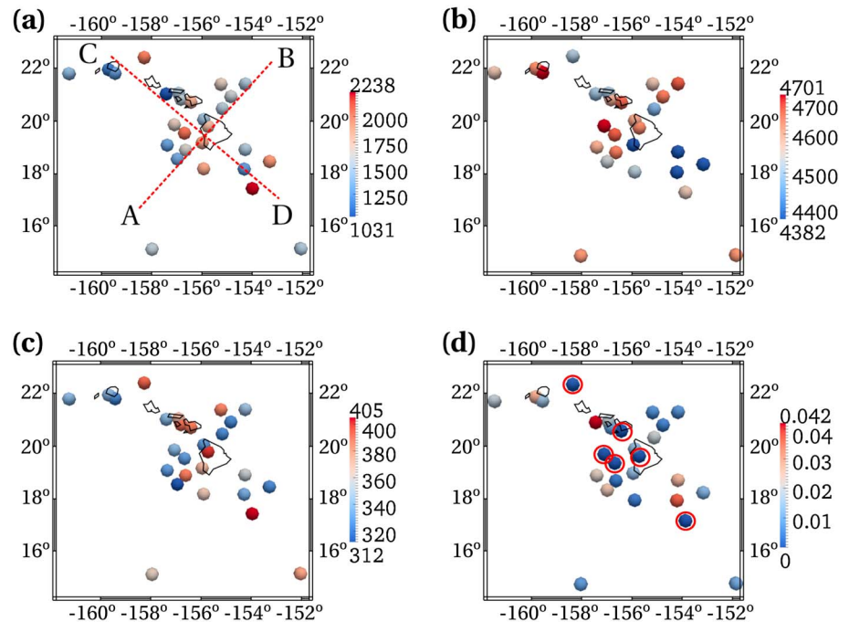
Figure 2. Maps of (a) calculated potential temperature, T , (b) observed seismic speed V_s^{obs} , (c) observed depth to the top of the LVL, and (d) calculated melt volume fraction beneath Hawaiian seismic stations. Each sphere is centered at the station location. The color of each sphere corresponds to the magnitude of the quantity according to the adjacent color scales. The spheres enclosed within red circles in Figure 2d register zero melt volume fraction. The results correspond to a dihedral angle of 10^\circ , basalt fraction of 0.2, and a reference potential temperature of 1800 K. The regionally averaged melt volume fraction from the map in Figure 2d is 1.1 \pm 0.8 vol%.
