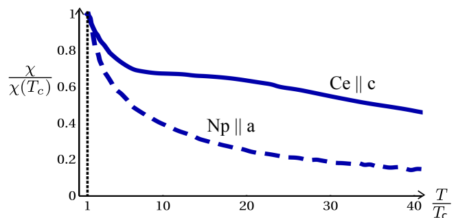
FIG. 1. Local moments are seen in the Curie-Weiss susceptibilities: CeCoIn 5 ( T_c = 2.3K ) 11 and NpPd 5 Al 2 ( T_c = 4.9K ) 3 are reproduced and rescaled by \chi(T_c) to show their similarity (data below T_c not shown).
