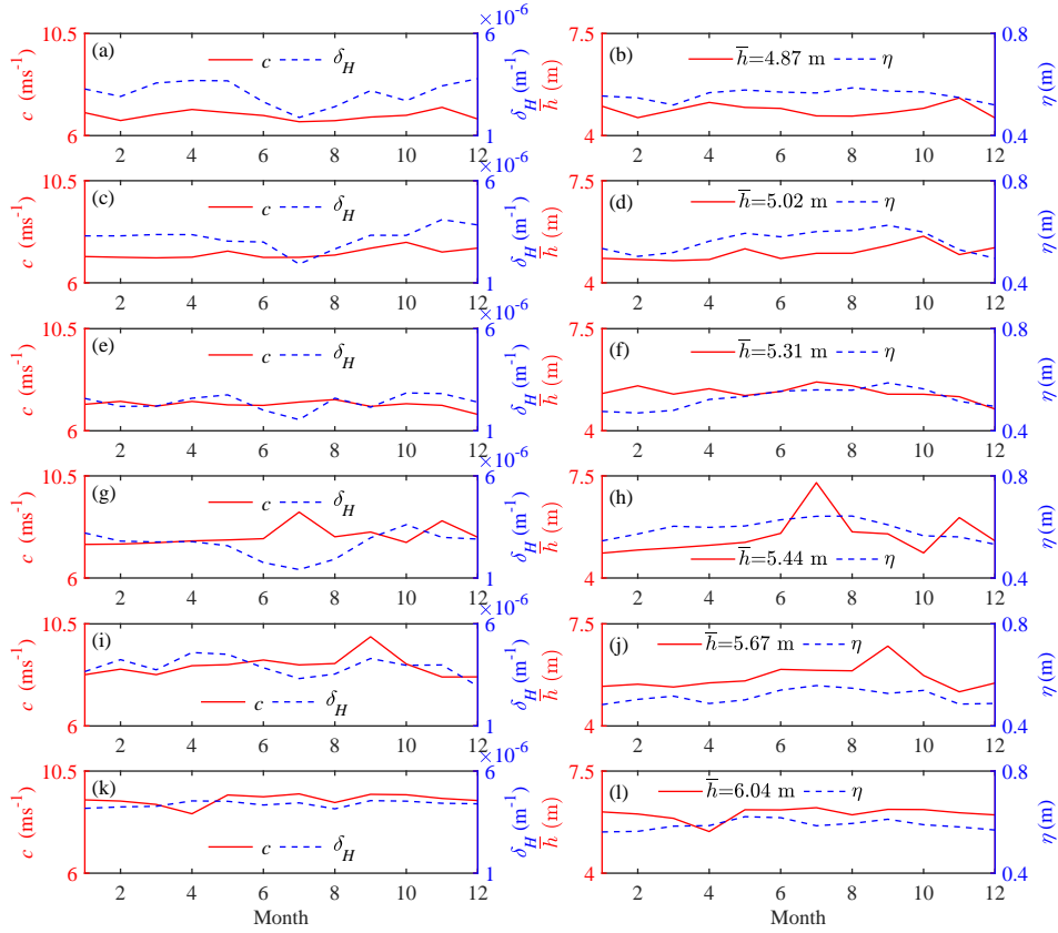
Fig. 11. Estimation of the tidally averaged depth \bar{h} (the right panels, together with the tidal amplitude at the CW station \eta ) using observed wave celerity c and tidal damping/amplification rate \delta_H (the left panels) for different years: 1965 (a, b), 1974 (c, d), 1989 (e, f), 1998 (g, h), 2009 (i, j) and 2015 (k, l).
