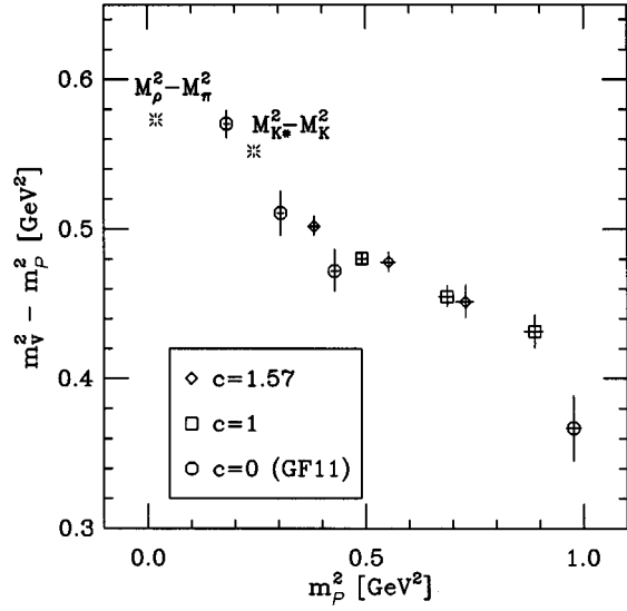
FIG. 9. The hyperfine splitting m_V^2 - m_P^2 versus m_P^2 for all the three values of c at \beta=5.7 , 16^3 \times 32 .
