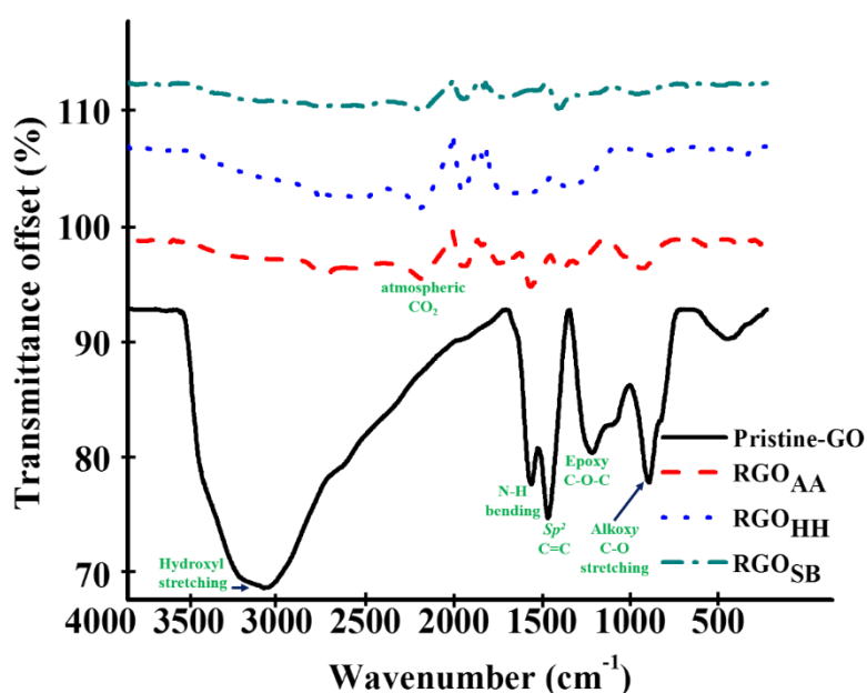
Fig. 6.3. ATR spectra of pristine-GO and RGO samples (reduced by means of ascorbic acid, hydrazine hydrate and sodium borohydride, respectively) restacked to avoid spectral overlap.
