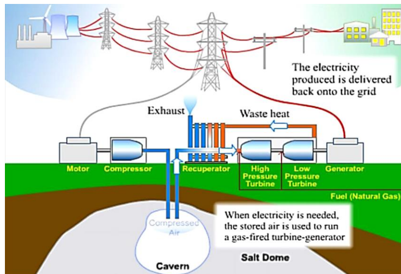
Fig. 1.1. Compressed air energy storage system [1.4].
