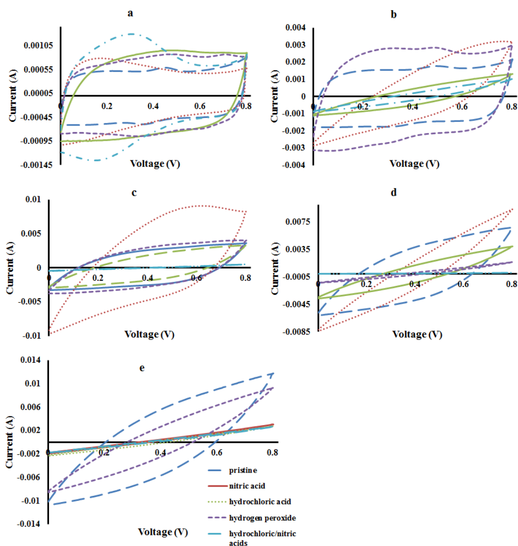
Figure 5.8. Cyclic voltammetry curves at scan rate of (a) 10, (b) 25, (c) 50, (d) 100 and (e) 200 mV s^{-1} using sodium sulfate as electrolyte.
