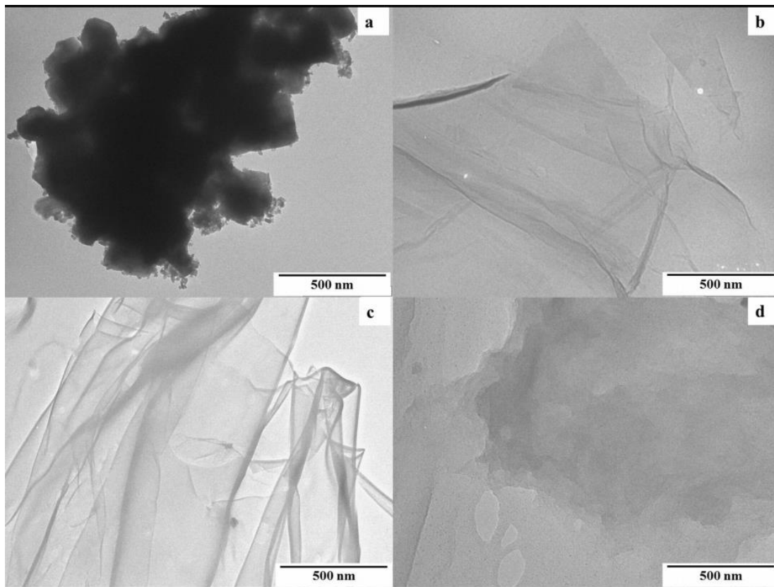
Fig. 4.1 TEM images for (a) graphite and GO samples from (b) G2N1-t 12,24 , (c) G1N1-t 12,24 and (d) G1N2-t 12,24 .
