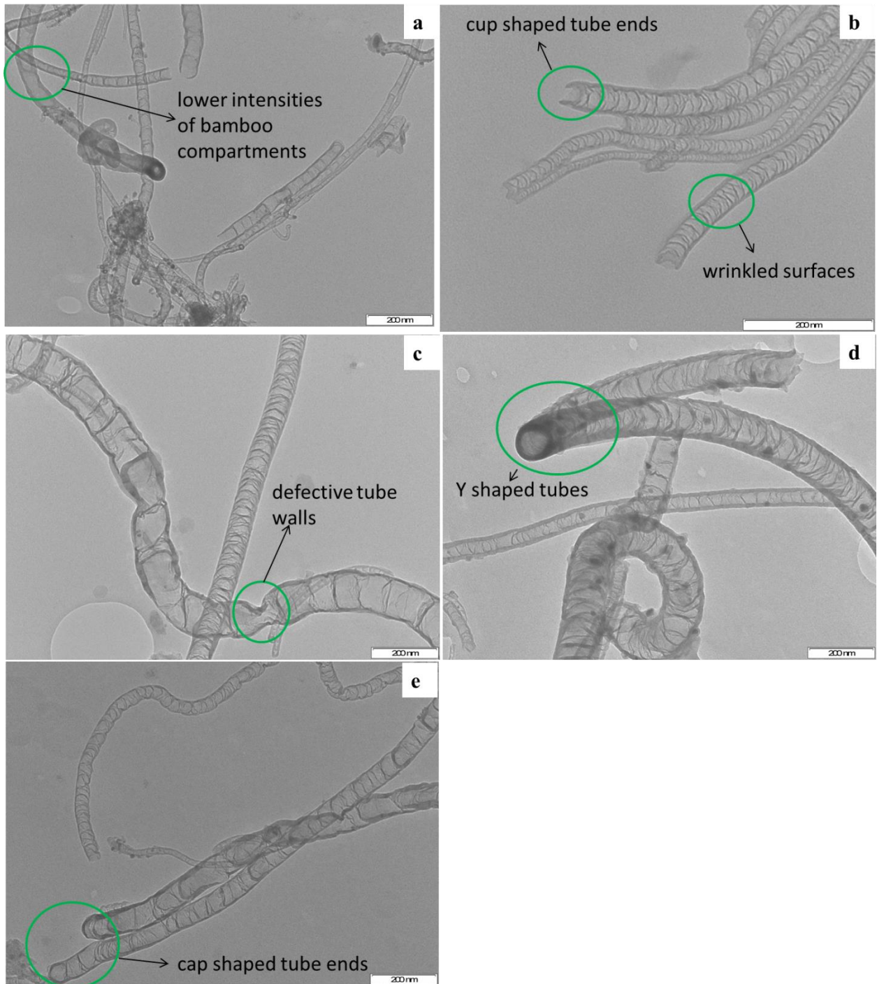
Fig. 3.19. The representative TEM images for the D1A3 samples (a) 800 °C, (b) 850 °C, (c) 900 °C, (d) 950 °C and (e) 1000 °C.
