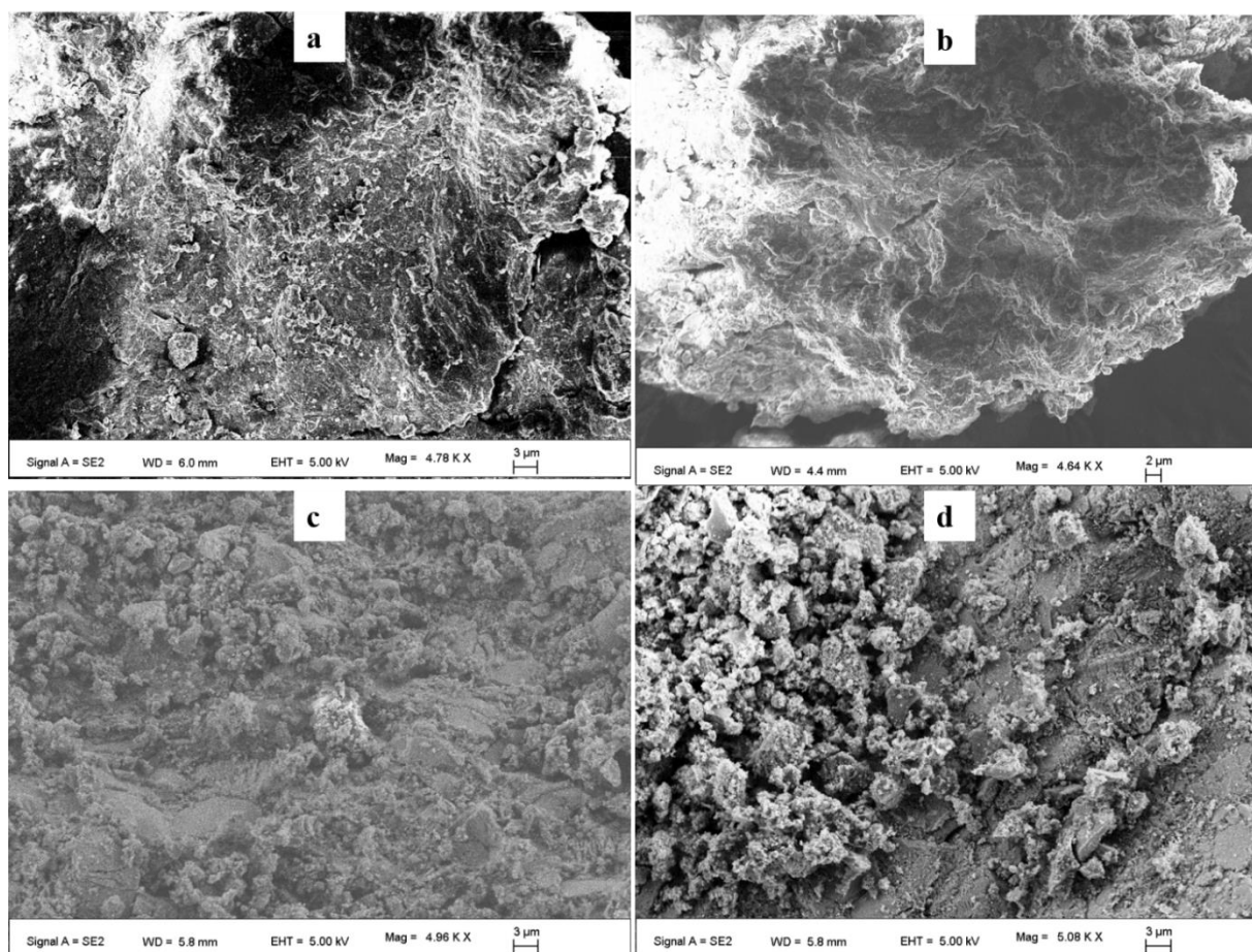
Fig. 7.4 SEM images of GOTi composites at titania wt.% of (a) 5%, (b) 10%, (c) 20% and (d) 40%
