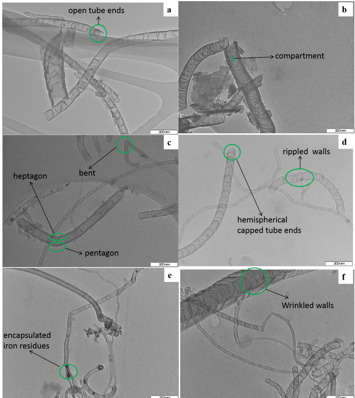
Fig. 3.5. The representative TEM images for the DxAl samples (a) D0A1, (b) D1A1, (c) D2A1, (d) D3A1, (e) D4A1 and (f) D5A1.
