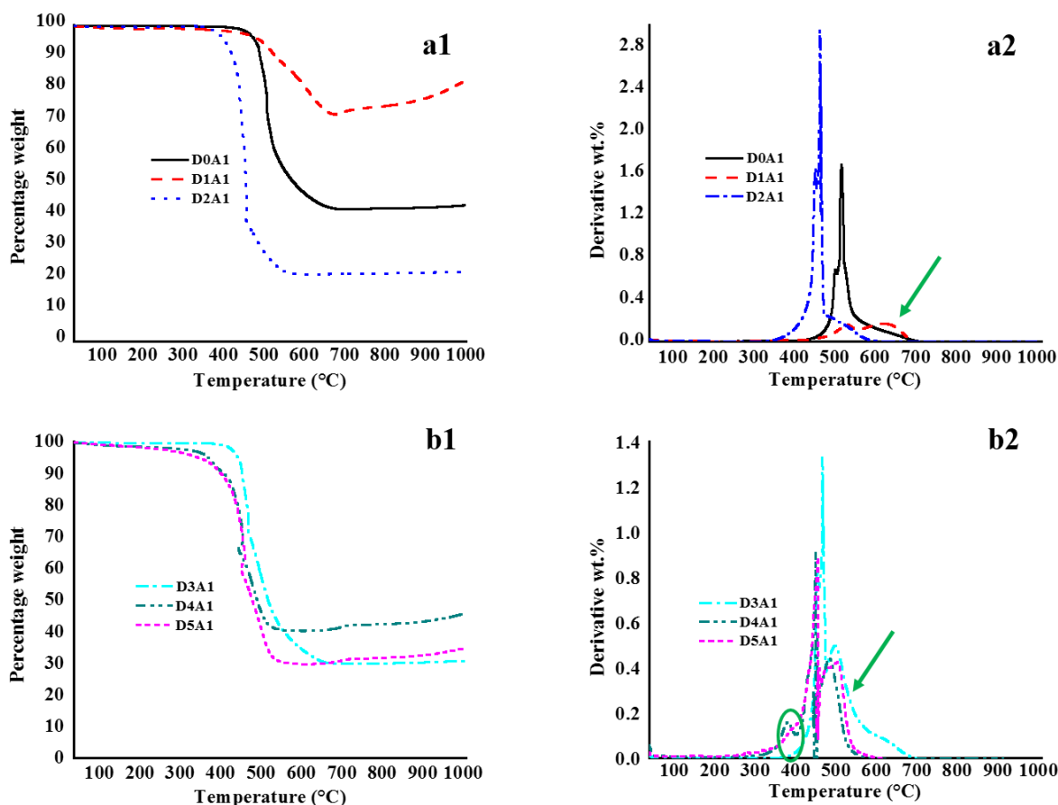
Fig. 3.6. Representative TGA (a1 and b1) thermograms and (a2 and b2) derivative weight curve for the DxA1 samples.
