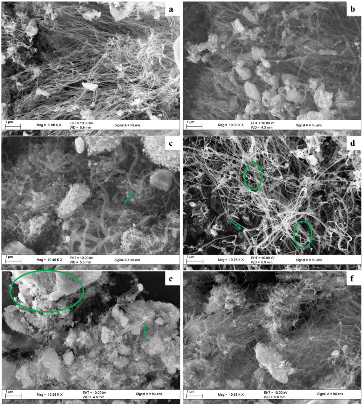
Fig. 3.4. The representative SEM images for the DxA1 samples (a) D0A1, (b) D1A1, (c) D2A1, (d) D3A1, (e) D4A1 and (f) D5A1.
