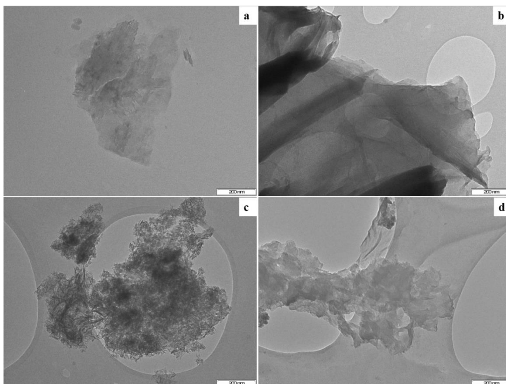
Fig. 6.4. TEM images for (a) pristine-GO, (b) RGO AA , (c) RGO HH and (d) RGO SB .
