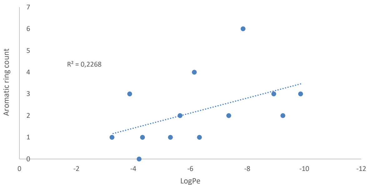
Figure 3.7: The relationship between the aromatic ring count for each test compound and effective permeability. There is a weak relationship between the effective permeability and the number of aromatic rings in each compound. There is no significant correlation between the aromatic ring count and the effective permeability ( p = 0.05 ), < 0.95 .
