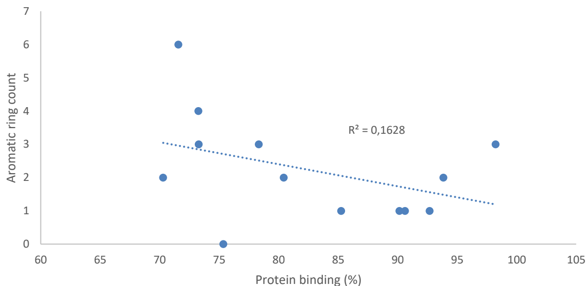
Figure 3.12: The percentage protein binding of the test compounds against the number of aromatic rings in each chemical compound structure. The low regression coefficient ( R^2 = 0.1628 ) above, is indicative of a weak relationship between the protein binding of compounds and the number of aromatic rings in each chemical compound. The weak relationship implies that each parameter is independent of each other.
