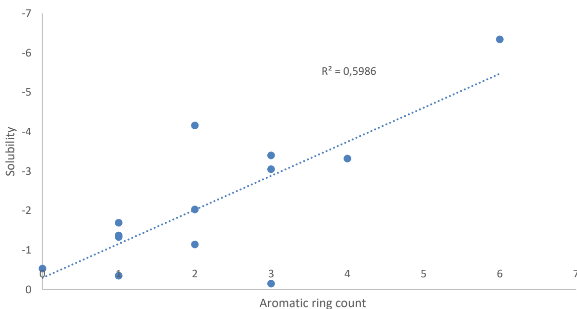
Figure 3.3: Relationship between the aromatic ring count and solubility of chemical compounds.
