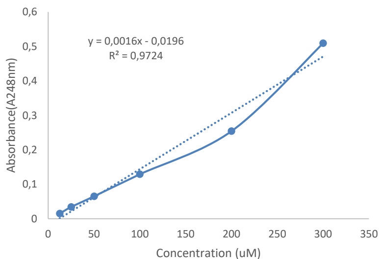
Figure 3.6: Caffeine (A), aniline (B), colchicine (C) and salicylic acid (D) standard curve constructed at different concentrations at specific wavelengths.
