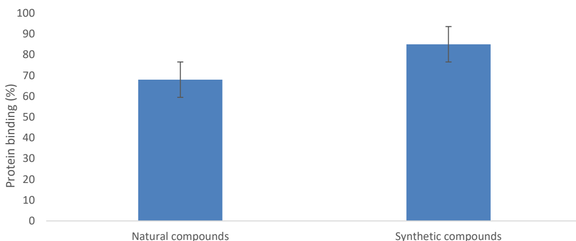
Figure 3.11: The difference between natural compounds and synthetic compounds based on their percentage protein binding. The above is the calculated average percentage protein-binding for a group of natural compounds and a group of synthetic compounds. There was a difference between natural compounds and synthetic compounds in terms of their average percentage protein-binding. Natural compounds displayed a lower average percentage protein-binding (67.98%) whilst the synthetic compounds displayed a higher average percentage protein-binding (85.01%).
