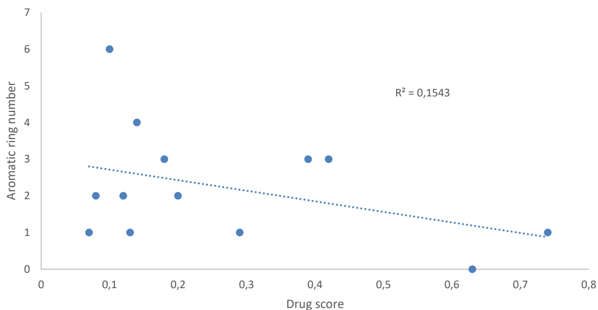
Figure 3.1: The relationship between the aromatic ring number of each compound and their corresponding drug score generated through Osiris Property Explorer. The correlation coefficient value of 0.1543 represents a weak relationship between the aromatic ring count and drug score. There is a significant difference between the aromatic ring count and the chemical compound's drug score ( p = 0.05 ).
