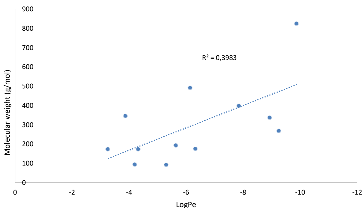
Figure 3.9: Relationship between molecular weight and \text{LogP}_e of the experimental compounds.
