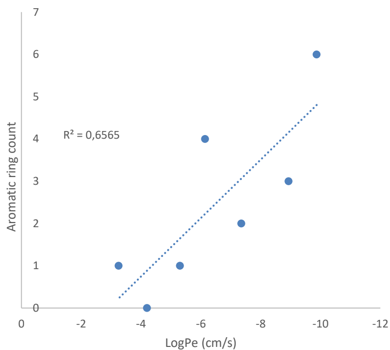
Figure 3.8: Relationship between the effective permeability and the number of aromatic rings for natural compounds (A) and synthetic compounds (B) structure. There is no true relationship between the effective permeability of natural compounds and the number of aromatic rings as indicated by the correlation coefficient of 0.0285 (A). A relationship exists between the effective permeability of synthetic compounds and the number of aromatic rings displaying a correlation coefficient of 0.6565 (B) as indicative of a positive correlation between the two parameters.
