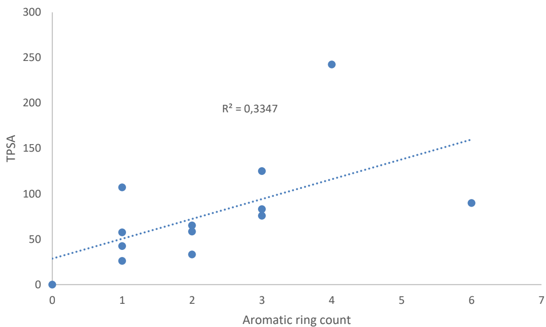
Figure 3.5: Relationship between the aromatic ring count and TPSA score generated through the Osiris Property Explorer. The regression coefficient value of 0.3347 is an indicative of a positive but weak and insignificant correlation between the aromatic ring count and TPSA ( p = 0.05 ) < 0.95 . Overall TPSA scores were low, with most points falling below 150, ranging from 150 to 45, implying the ease of absorption of the chemical compounds.
