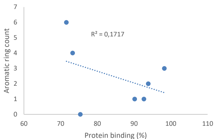
Figure 3.13: Relationship between the percentage protein-binding and the number of aromatic rings for natural compounds (A) and synthetic compounds (B). A true relationship between percentage protein-binding and aromatic ring number on a group of natural compounds, with a correlation coefficient of 0.8364 whilst synthetic compounds displayed a weak relationship between the aromatic ring count and percentage protein-binding.
