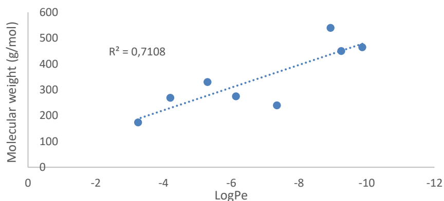
Figure 3.10: The relationship between the effective permeability and molecular weight of natural compounds (A) and synthetic compounds (B). There is a positive correlation between the molecular weight and the LogP e of both, the natural compounds and synthetic compound group. A relationship between the molecular weight and LogP e of natural compounds produced a correlation coefficient value of 0.245 which was significantly ( p > 0.05 ) lower than the correlation coefficient value of 0.7108 produced from the relationship between the molecular weight and LogP e of synthetic compounds.
