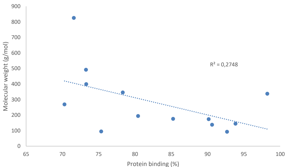
Figure 3.14: Relationship between the percentage protein-binding and molecular weight. Percentage protein-binding for all test compounds was above 60% as indicated here hence all points congested in a range 60-100 %. Even so, there was a weak relationship between molecular weight and percentage protein binding observed, this is indicated by the correlation coefficient value 0.2748. Each of the two parameters is independent of the other. There is an upward trend but this is just a trend rather than a statistically validated correlation.
