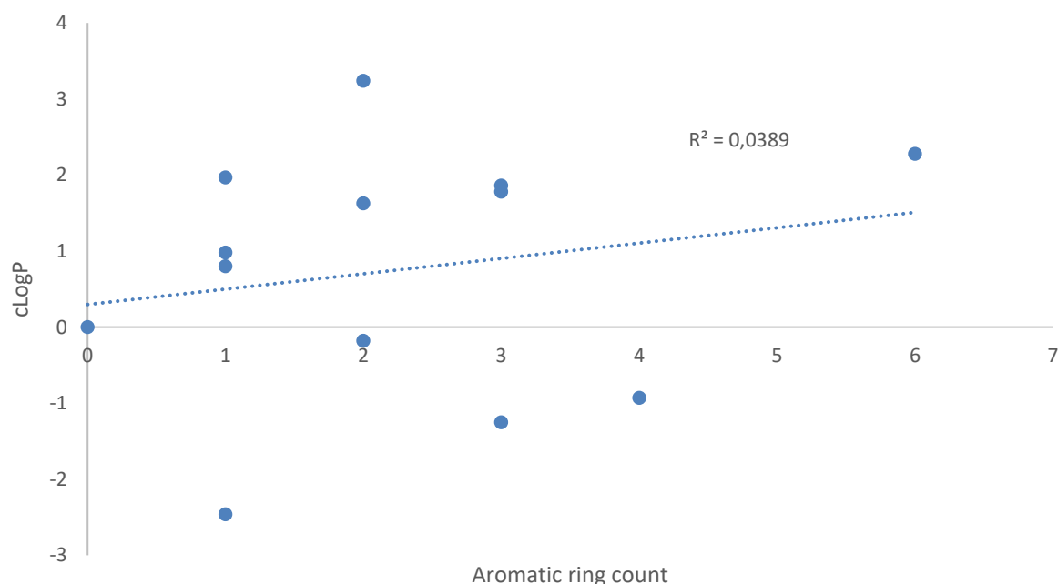
Figure 3.2: Relationship between the lipophilicity of chemical compounds and the aromatic ring count. A weak relationship was observed between lipophilicity and aromatic ring count indicated by the low correlation coefficient value of 0.0389. According to Lipinski's Rule of Five, lipophilicity values of compounds intended for oral administration should be less than 5.00. There is a significant difference between the aromatic ring count and lipophilicity of chemical compounds ( p = 0.05 ).
