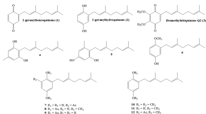
Figure 1. Structure of some active linear geranylquinone and geranylphenols.
