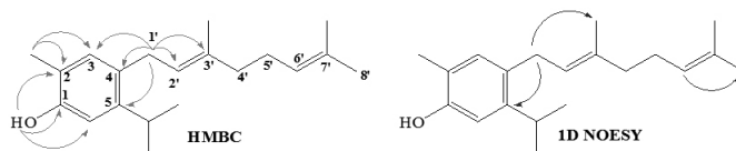
Figure 8. Main 2D ^1\text{H} - ^{13}\text{C} HMBC and 1D NOESY observed correlations in the NMR experiments for the compound 20 , these confirm the aromatic substitution position and geometrical orientation of double bond in the geranyl chain.
