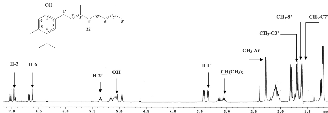
Figure 10. ^1\text{H} NMR spectrum of the mixture compounds 21/22 and identification of the signals corresponding to the compound 22 .
