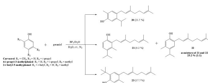
Scheme 3: Synthetic route for the obtaining of derivatives 20-23 by direct geranylation reaction between, carvacrol, 4- i -propyl-3-methylphenol and 2- t -butyl-5-methylphenol and geraniol in \text{Et}_2\text{O} catalyzed by \text{BF}_3 \cdot \text{Et}_2\text{O} .
