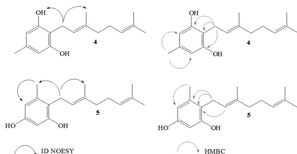
Figure 3. Observed correlations 1D NOESY and 2D ^1\text{H} - ^{13}\text{C} HMBC in the NMR experiments for the compounds 4 and 5 , which confirm the position and geometrical orientation of double bond in the geranyl chain.
