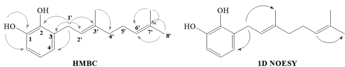
Figure 7. Principal 2D ^1\text{H} - ^{13}\text{C} HMBC and 1D NOESY observed correlations in the NMR experiments for the compound 19 , these confirm the aromatic substitution position and geometrical orientation of double bond in the geranyl chain.
