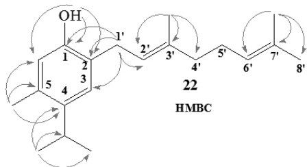
Figure 11. Major 2D ^1\text{H} - ^{13}\text{C} HMBC observed correlations in the NMR spectrum for the compound 22 .
