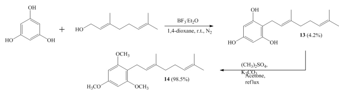
Scheme 1: Synthesis of geranylphloroglucinol 13 and their trimethoxylated derivative 14 .
