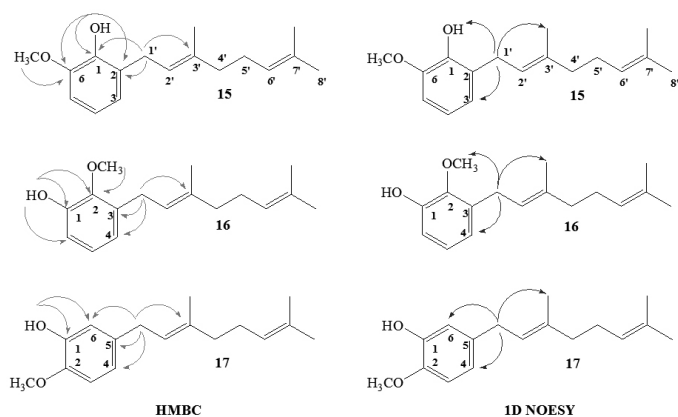
Figure 5. Main 2D HMBC and 1D NOESY observed correlations that allowed differentiate and determine the regio-isomer structures 15 , 16 and 17 .
