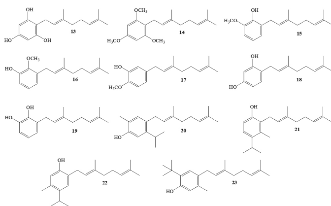
Figure 2. Structure of new linear geranylphenol derivatives.
