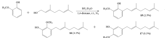
Scheme 2: Synthesis of derivatives 15 , 16 and 17 by direct geranylation between geraniol and guaiacol (2-methoxyphenol) catalyzed by \text{BF}_3 \cdot \text{Et}_2\text{O} .
