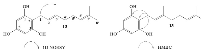
Figure 4. Observed correlations 1D NOESY and 2D ^1\text{H} - ^{13}\text{C} HMBC in the NMR experiments for the compound 13 , which confirm the position and geometrical orientation of double bond in the geranyl chain.
