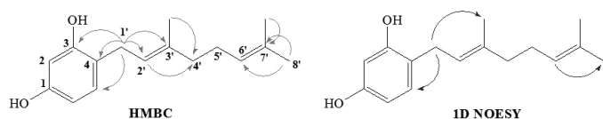
Figure 6. 2D ^1\text{H} - ^{13}\text{C} HMBC and 1D NOESY observed correlations in the NMR experiments for the compound 18 , which confirm the aromatic substitution position and geometrical orientation of double bond in the geranyl chain.
