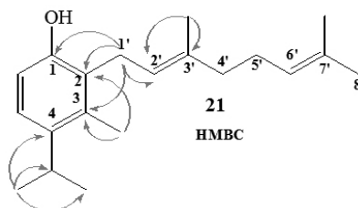
Figure 9. Main 2D ^1\text{H} - ^{13}\text{C} HMBC observed correlations in the NMR spectrum for the compound 21 , which confirm the aromatic substitution position of the geranyl chain.
