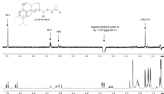
Figure 12. Bottom: normal ^1\text{H} -NMR spectrum of mixture 21/22 ; Top: selective gs 1D NOESY irradiation at \delta = 3.35 ppm for compound 22 in the mixture, which long-range interactions can clearly be seen between H-1' with H-3, OH, H-2' and \text{CH}_3\text{-C}3' .
