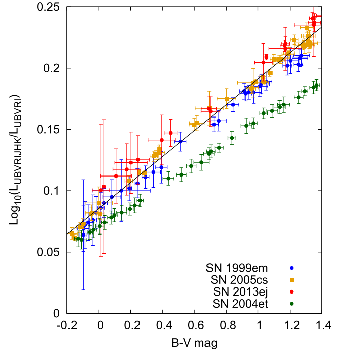
Figure 14. Linear behavior of the log of the ratio of flux with B - V . A tight correlation of \log_{10}(UBVR IJHK/UBVRI) with B - V is seen for SNe 1999em, 2005cs, and 2013ej. The fit has \chi^2/\text{dof} = 1.51 . The atypical SN IIP 2004et is shown and not included in the fit. The derived fit is given by Equation (2).
