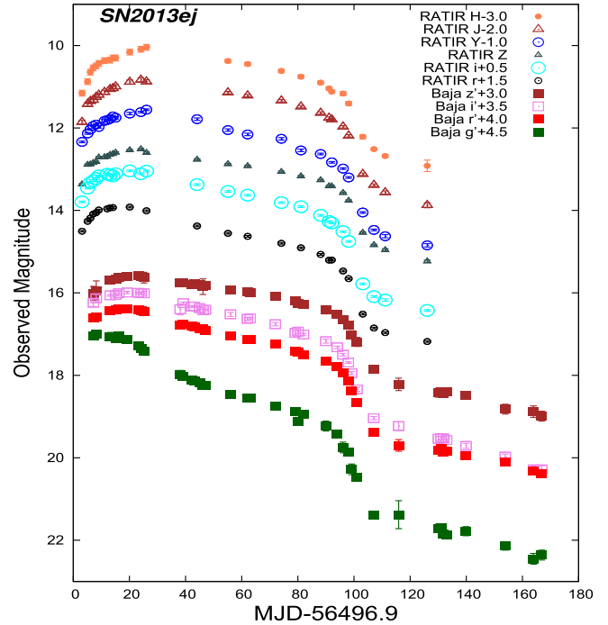
Figure 3. SDSS g'r'i'z' photometry from Baja Observatory, as well as RATIR optical and near-IR photometry, of SN 2013ej.
