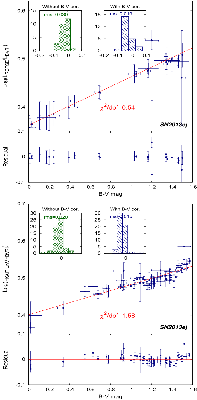
Figure 12. Top panel: pseudo-bolometric BVRI calibration of SN 2013ej from ROTSE unfiltered photometry compared to Konkoly BVRI photometry. Residual from a B - V color-dependent correction (histogram in blue) shows less than 5% uncertainty. The histogram shown on the left (green) is obtained from the residuals by comparing the two fluxes without any color correction. Bottom panel: same as in top panel, but for KAIT unfiltered to KAIT BVRI calibration. We obtain 6% residuals by direct comparison and 4% residuals when applying a B - V dependence. Fit equations for B - V dependence are given in Table 5.
