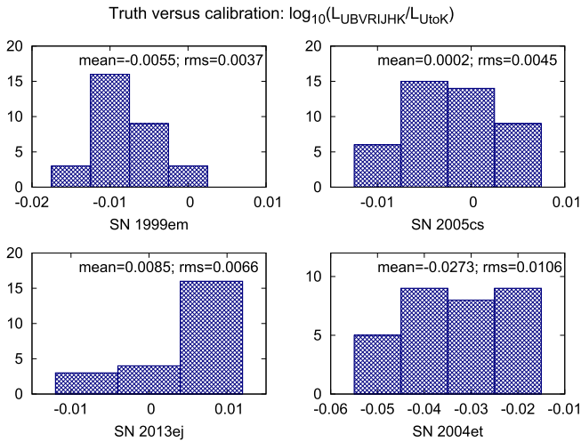
Figure 15. Histograms obtained after subtracting \log_{10}(L_{UtoK}/L_{UBVRI}) from \log_{10}(L_{UBVRIJHK}/L_{UBVRI}) . The mean and the rms of the difference confirm 1%–2% precision for SN 2013ej, SN 1999em, and SN 2005cs. Applying the same calibration to SN 2004et (not included in the fit) yields ~6% precision. Note that the values given in the figures are in \log_{10} .
