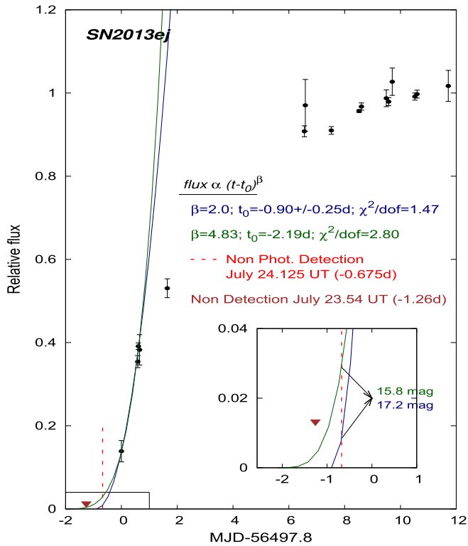
Figure 6. Early rise behavior of SN 2013ej. Multiple data sets calibrated to ROTSE magnitudes (see text) are shown. Solid lines are power-law fits to data obtained before +2 day since explosion. The triangle point is a nondetection limit on July 23.54 at V \approx 16.7 mag, shown here for reference. The dashed line indicates the detection on July 24.125 with no photometry available. The inset illustrates the projection of where the emission would be for floating index (green) and fixed index \beta = 2 (blue).
