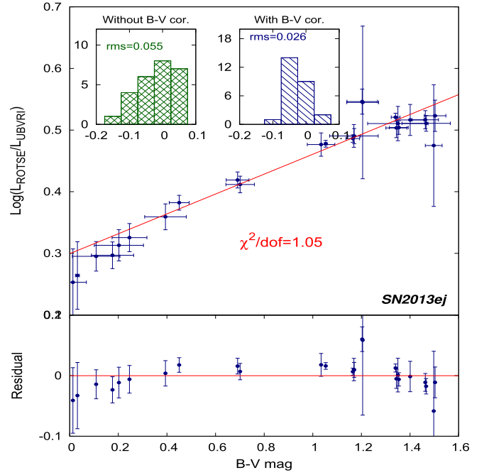
Figure 13. Pseudo-bolometric UBVR I calibration of SN 2013ej from the ROTSE luminosity. The B - V color-dependent correction (histogram in blue) improves the measurement by about a factor of 2 compared to direct comparison (histogram in green).
