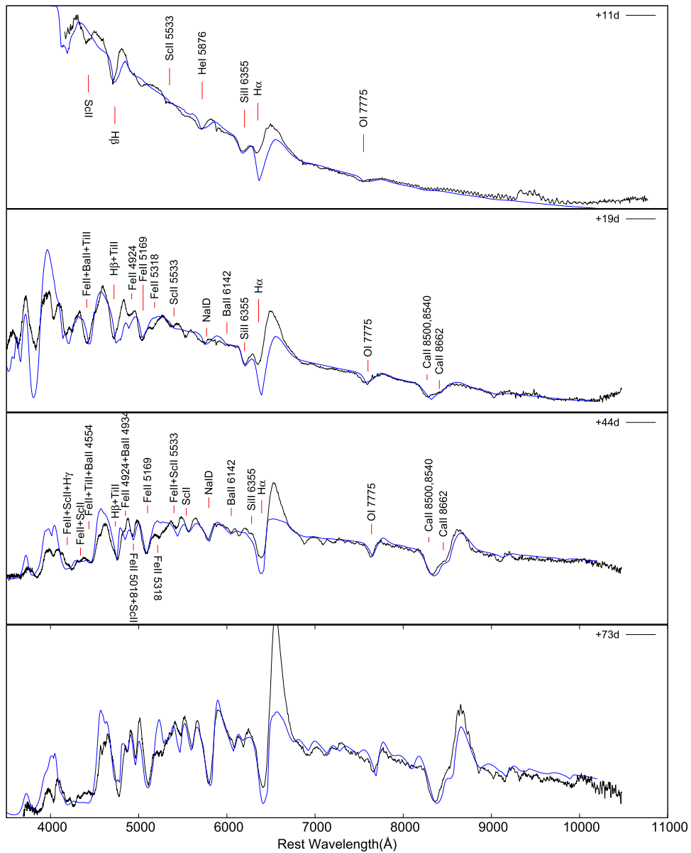
Figure 19. Example Syn++ fits of SN 2013ej spectra are shown in blue while data are in black. The fits mostly reproduce the observed features. The inability to accurately reproduce the H I line profile is perhaps a limitation of the model being purely scattering based and not accounting for the emission from recombination cascades and the NLTE effects. SN 2013ej exhibits most previously identified SN IIP spectral features.
