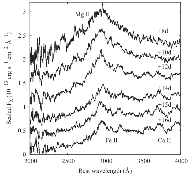
Figure 5. Spectral evolution of SN 2013ej in the UV based on Swift /UGRISM observations. Labels next to each spectrum indicate the days since explosion (MJD 56496.9). Feature identifications are based on Bufano et al. (2009).
