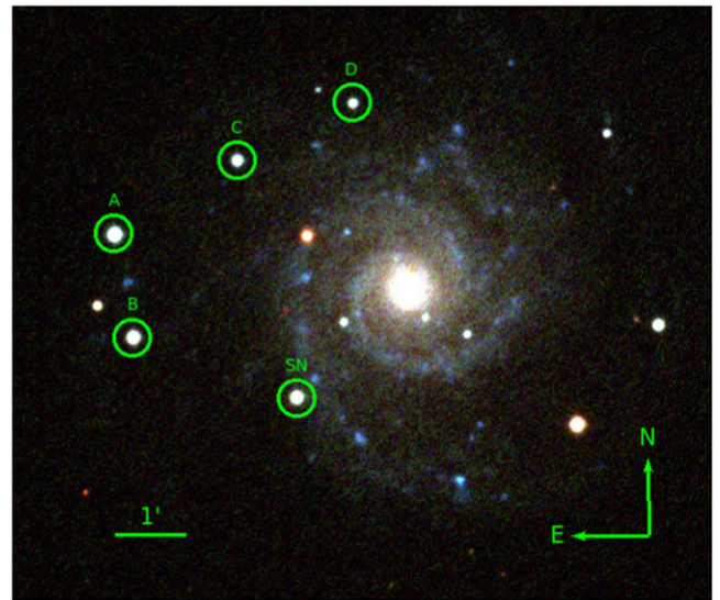
Figure 1. Field around SN 2013ej on a color-combined ( BVI ) CCD frame taken with the 0.6 m Schmidt telescope at Konkoly Observatory, Piszkesteto, Hungary. Konkoly photometry reference stars in the vicinity of SN 2013ej are shown.
