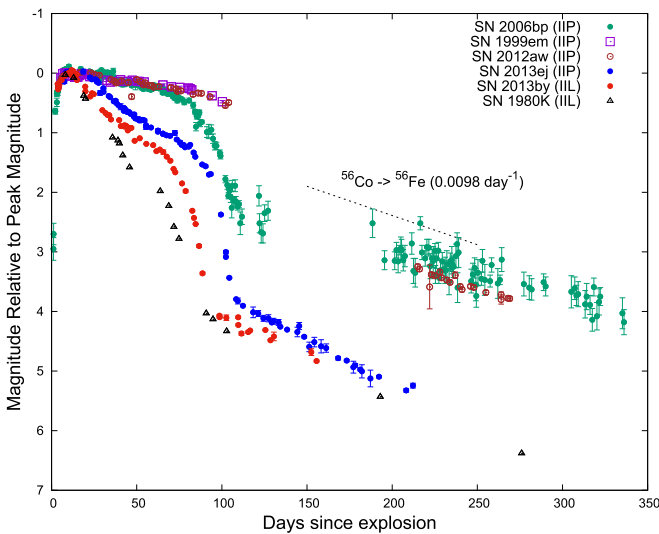
Figure 7. Comparison of some SN IIP and SN IIL light curves in the V band, except SN 2006bp (ROTSE). SN 2013ej has a systematically steeper plateau, with a sharp drop at the end of the plateau. SNe IIL 2013by and 1980K have steep linear evolution after peak, but the drop at the end of the plateau is not as sharp. SN 2013ej also exhibits a steeper tail decline than the events shown here.
