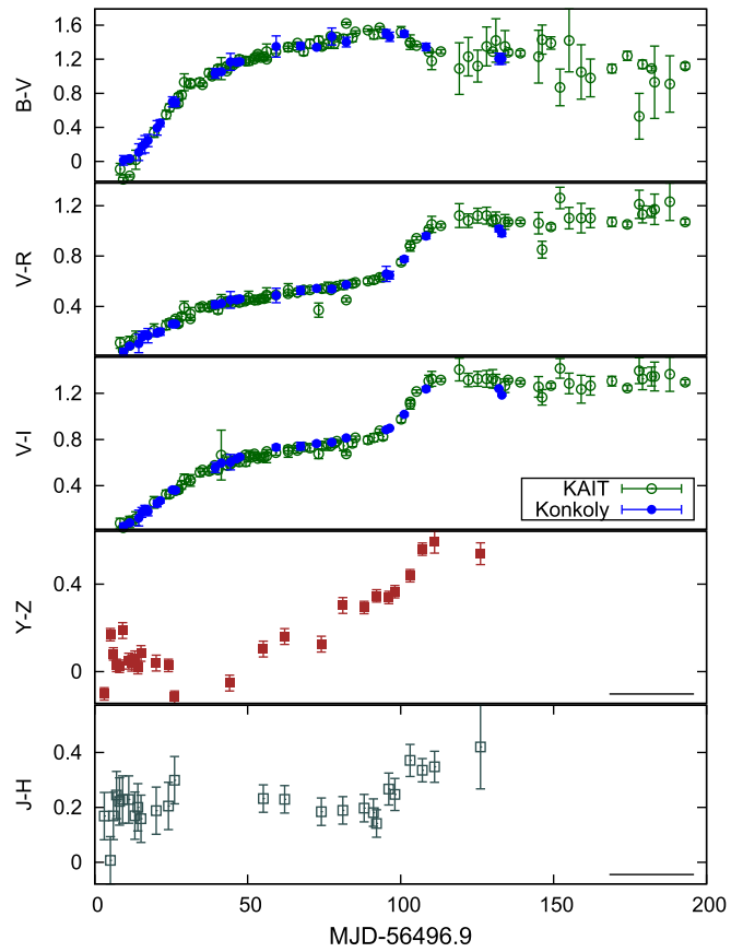
Figure 8. Optical and near-IR color evolution of SN 2013ej. Here, the J - H and Y - Z colors from RATIR are shown in the Vega system for consistency.
