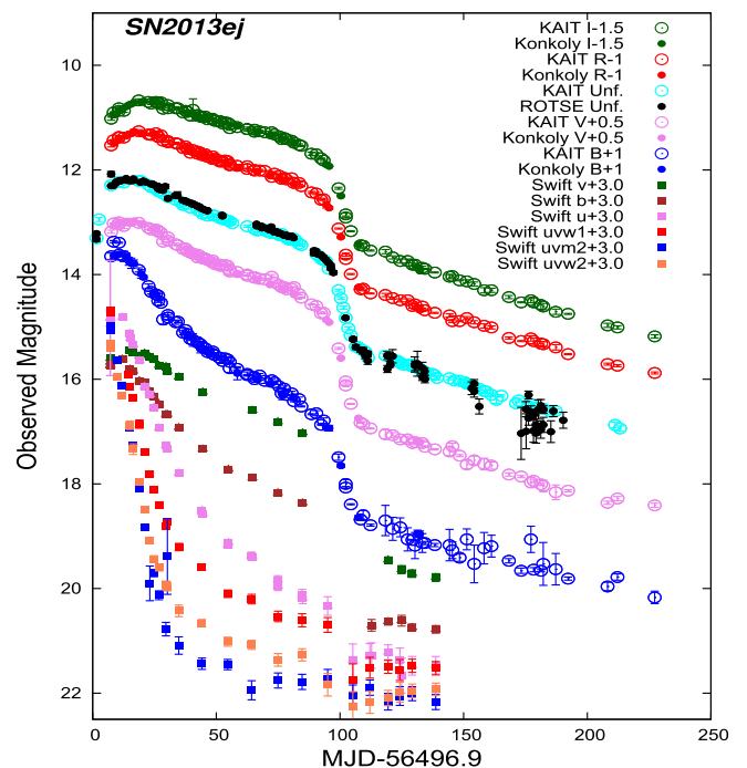
Figure 2. Open CCD and multiband photometry of SN 2013ej. KAIT BVI and unfiltered data points are shown with empty circles, while Konkoly BVI and ROTSE points are solid circles. Swift photometry is represented with filled square symbols.
