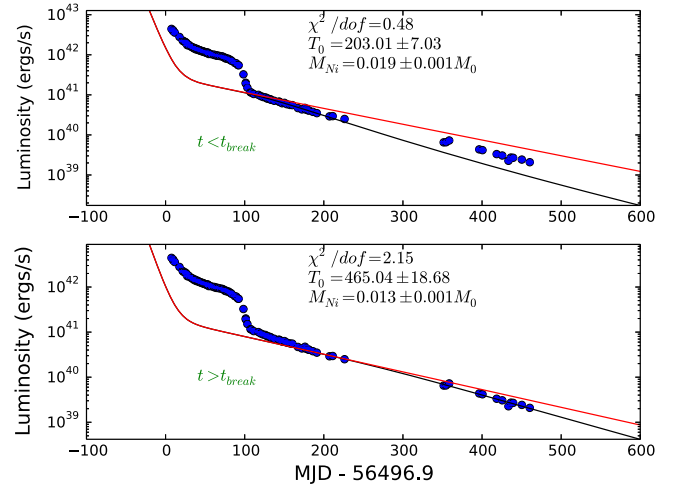
Figure 23. Fit of the radioactive decay model of Equation (11) to the bolometric light curve tail of SN 2013ej. Pre-break time and post break time lightcurves are fitted separately. The upper panel shows the fit taking data between +120 day and the break point at +183 day. The lower panel shows the same fit taking data beyond the break time. The leakage of both the gamma-rays and positrons were taken into account in the model (see text). The red line represents full trapping of gamma rays and positrons on both panels.
