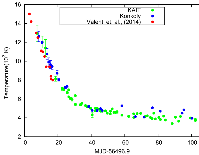
Figure 10. Evolution of the photospheric temperature using the KAIT (green points) and Konkoly (blue points) BVI data sets. Temperature estimates from Valenti et al. (2014) are shown with red points.
