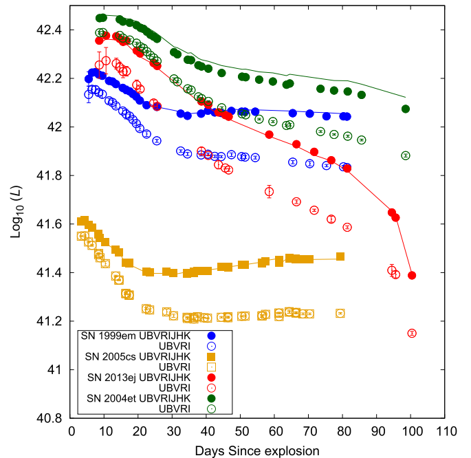
Figure 16. Comparison of calibrated luminosity with measured luminosity. Solid lines represent UtoK light curves while empty and solid circles represent UBVRI and UBVRIJHK light curves. While 1%–2% precision in the calibration is obtained for SN 2013ej, SN 2005cs, and SN 1999em, the outlier SN 2004et is also calibrated with about 6% precision.
