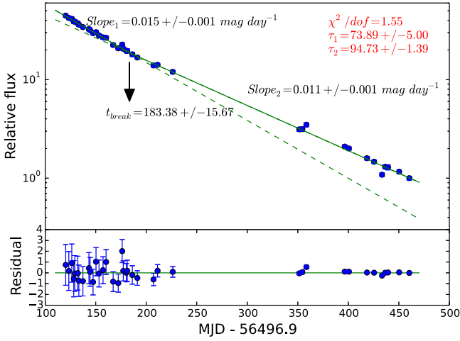
Figure 22. Fit of the bolometric light curve of SN 2013ej beyond +120 day with a broken exponential law. The solid line is the fitted model while the dashed lines are the extrapolation of each exponential models in either direction. The crossover is at break time, t_{br} = +183.4 \pm 15.7 day.
