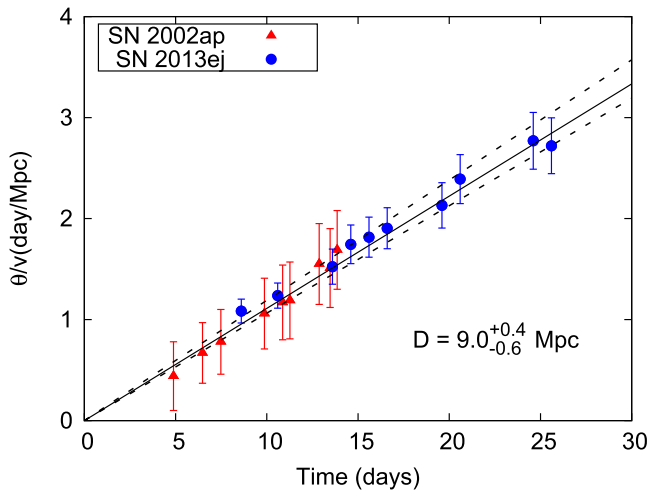
Figure 21. Distance measurement of M74 using SN 2013ej and SN 2002ap. The black solid line shows the final result that yields a distance of 9.0 Mpc, while the dotted lines mark its uncertainty.
