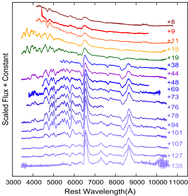
Figure 4. Time series of optical spectra of SN 2013ej. Phases are in days since explosion (MJD 56496.9). The log of observations is given in Table 2.
