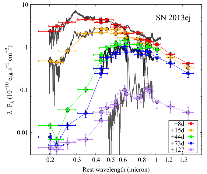
Figure 9. Evolution of the spectral energy distribution (SED) of SN 2013ej. Fluxes from broadband photometry from the UV, optical, and near-IR are plotted with filled circles, and the horizontal bars represent the FWHM of each filter. Phases are coded by colors and indicated in the legends. The optical and UV spectra at certain epochs (where available) are also overplotted for comparison. Dereddening with E(B - V) = 0.061 mag has been applied.
