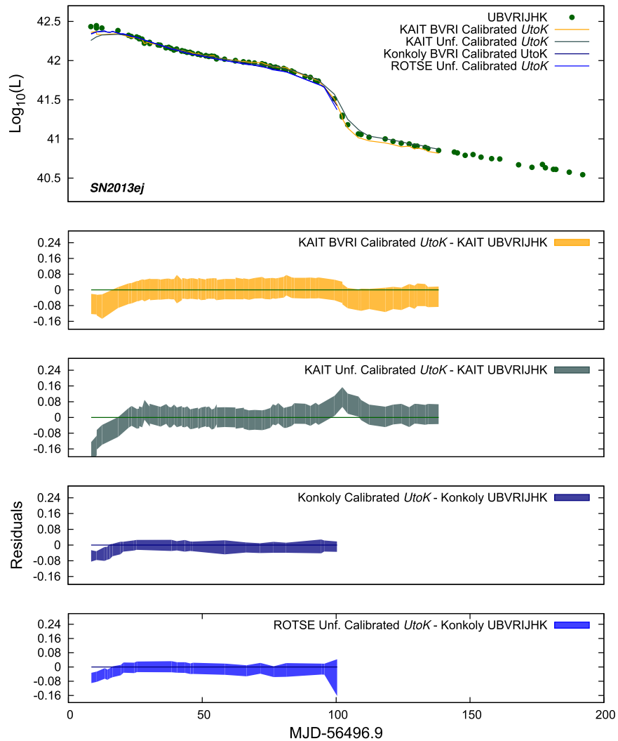
Figure 17. UtoK luminosity obtained from calibrating broadband and unfiltered photometry from KAIT, Konkoly, and ROTSE data for SN 2013ej. Data points UBVR IJHK in the top panel are integrated U from Swift , KAIT BVRI , RATIR JH , and an estimated K flux (see text). Shaded regions in the residual plots indicate 1\sigma uncertainty from the rms of the residuals. For KAIT data, we have added systematic uncertainty based on the differences of KAIT UBVR IJHK and UtoK values derived from UBVR I luminosity using Equation (2), which is derived using Konkoly data. The highest offset at very early times is a result of the high UV contribution to the total flux.
