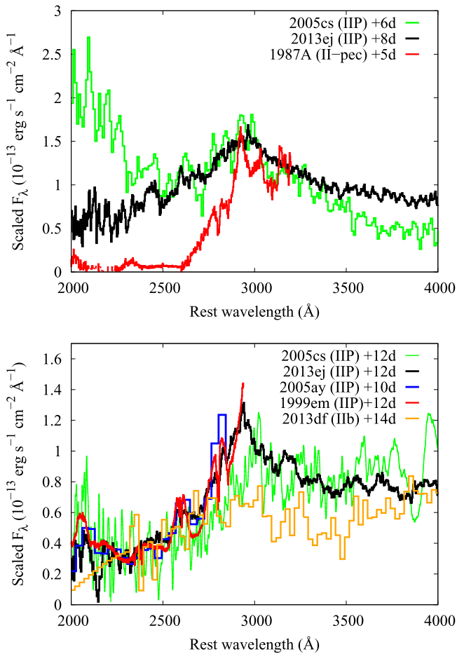
Figure 18. Evidence of spectral homogeneity of SNe IIP in the UV at early times. Top panel: SN 2013ej UV spectrum compared with the atypical SN 1987A, which shows a sharp UV cutoff, while the excess flux of SN 2005cs below 2500 Å is suspected to be coming from a different source. Bottom panel: homogeneous SN IIP UV sample at \sim 12 day. Also shown for comparison is a SN Iib spectrum, which is clearly distinct from the rest.
