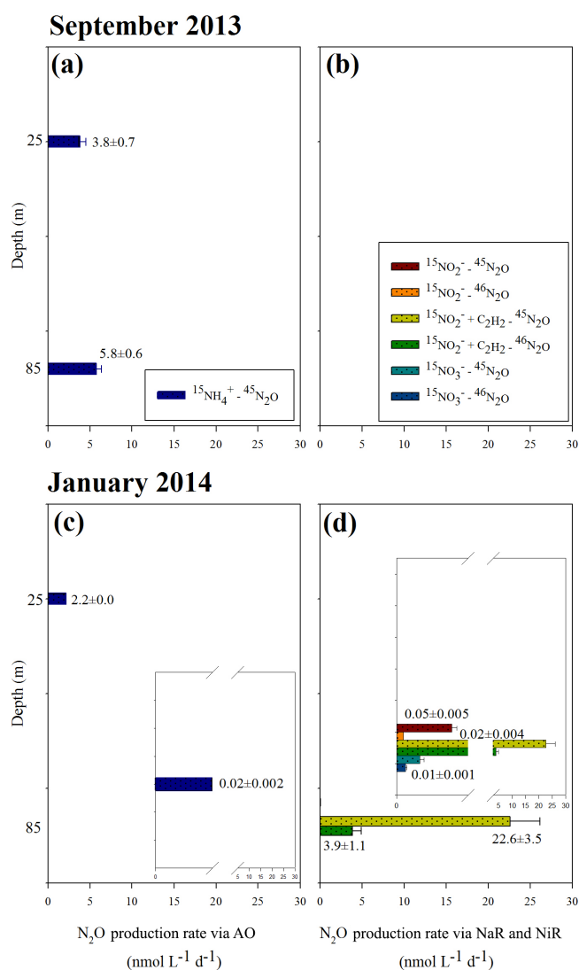
Figure 4. \text{N}_2\text{O} production rates through AO (a, c), and through NaR and NiR (b, d) measured in the oxycline (25 m depth) and bottom layer (85 m depth) at Sta. 18 over the continental shelf off central Chile during 12 September 2013 (a, b) and 28 January 2014 (c, d). Conventions show the amended tracer ( ^{15}\text{NH}_4^+ , ^{15}\text{NO}_2^- , and ^{15}\text{NO}_3^- ), isotopic pairing in the gas produced, and inhibitor when used (acetylene – “ \text{C}_2\text{H}_2 ”). Note that \text{N}_2\text{O} produced in the incubations with \text{C}_2\text{H}_2 represents gross production rates. Insets in (c) and (d) represent details of lower values at depth.
