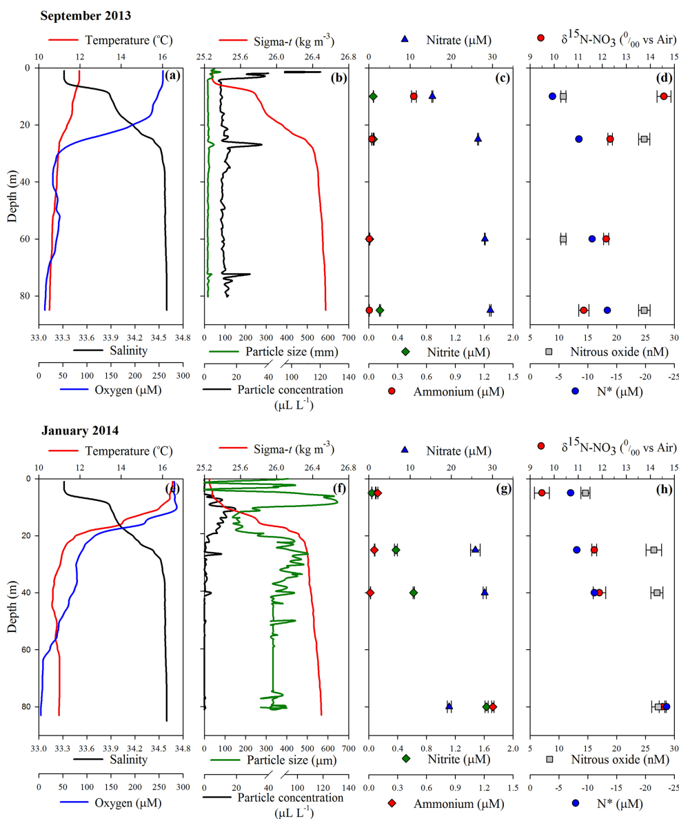
Figure 2. Water column profiles of hydrographic parameters during sampling periods (a–d, 12 September 2013 and e–h, 28 January 2014) at station 18 over the continental shelf off central Chile.
