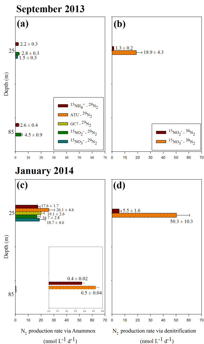
Figure 3. Anammox (a, c) and denitrification (b, d) activities expressed as \text{N}_2 production rates measured in the oxycline (25 m depth) and bottom layer (85 m depth) at Sta. 18 over the continental shelf off central Chile during 12 September 2013 (a, b) and 28 January 2014 (c, d). Conventions show the amended tracer ( ^{15}\text{NH}_4^+ , ^{15}\text{NO}_2^- , and ^{15}\text{NO}_3^- ), isotopic pairing in the gas produced, and inhibitor when used (ATU and GC7). Inset in (c) represents details of lower values at depth.
