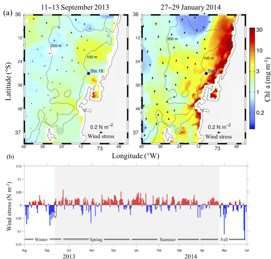
Figure 1. (a) Satellite-derived chlorophyll- a and wind stress during the period around the sampling days (left panel spring transition and right panel summer), for the study area and location of time series station 18 (Sta. 18; blue dot; 36°30' S; 73°08' W) off central Chile, Concepción Bay. (b) Upwelling- (red bars) and downwelling-favourable (blue bars) alongshore wind stress related to the study period (August 2013–May 2014). Box plots represent the statistical values boundaries of wind stress data for the previous week (5 days) to each sampling time. Part of the box closest and farthest to zero are the 25th and 75th percentile, respectively; horizontal lines within the box are the mean; and whiskers (error bars) are the minimum and maximum values. Shaded area represents the upwelling season.
