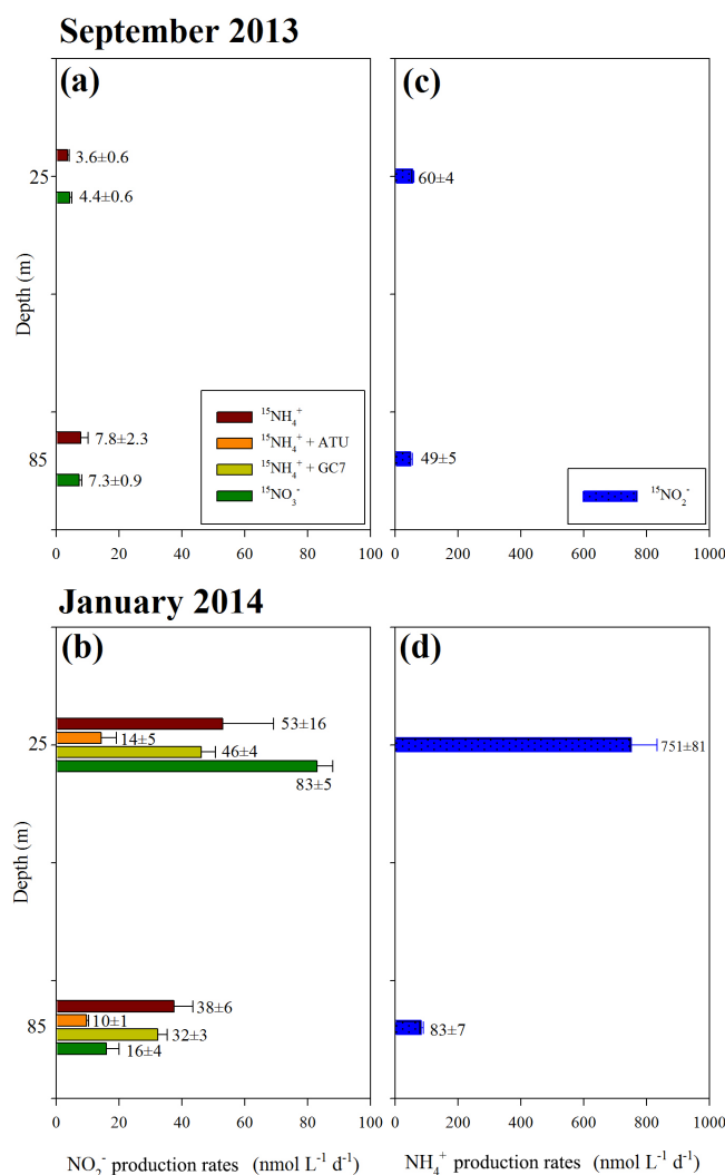
Figure 5. Nitrite (a, b) and ammonium (c, d) production rates measured as ^{15}\text{N}_2 after chemical conversion of the dissolved ^{15}\text{N} -inorganic compound produced (formed by redox reactions) measured in the oxycline (25 m depth) and bottom layer (85 m depth) at Sta. 18 over the continental shelf off central Chile during 12 September 2013 (a, c) and 28 January 2014 (b, d). Conventions denote amended tracer/source ( ^{15}\text{NH}_4^+ , ^{15}\text{NO}_3^- , and ^{15}\text{NO}_2^- ) and inhibitor (ATU and GC7) that showed activities.
