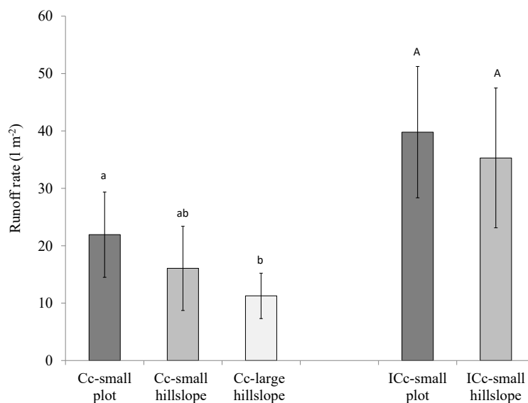
Figure 5. Total runoff rates during the period shown in Table 2 (26 January–21 March 2010) in well-developed cyanobacterial (Cc) and incipient-cyanobacterial (ICc) biocrusts at El Cautivo, at plot ( \sim 10 m 2 ), small-hillslope ( \sim 10 m 2 ) and large-hillslope ( \sim 20 m 2 ) scales. There were no plots at large-hillslope scale for the ICc crust. Different letters indicate significant differences ( p < 0.05 ) among spatial scales for each crust type.
