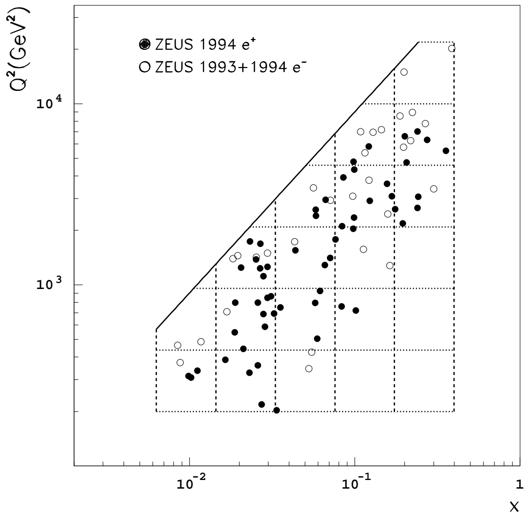
Figure 1: Distribution of events in the (x, Q^2) plane. The filled (open) circles indicate the selected e^+p ( e^-p ) CC events in a sample with integrated luminosity of 2.93 \text{ pb}^{-1} ( 0.82 \text{ pb}^{-1} ). The horizontal lines of the grid show the Q^2 , the vertical lines the x bins used for the analysis. The solid diagonal line indicates the kinematic limit y = 1 .
