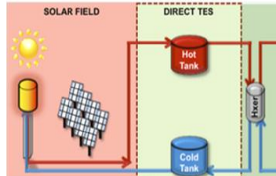
Figure 12. Two-tanks direct TES system integrated into a CSP plant [21]
