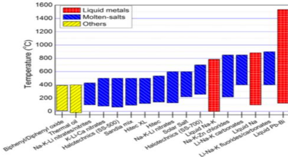
Figure 10. Operating temperature range for various HTFs [5].
