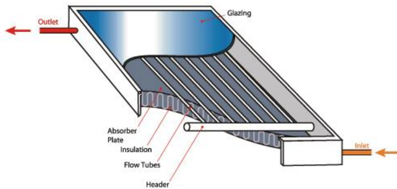
Figure 3. Schematic view of an FPC [6].
