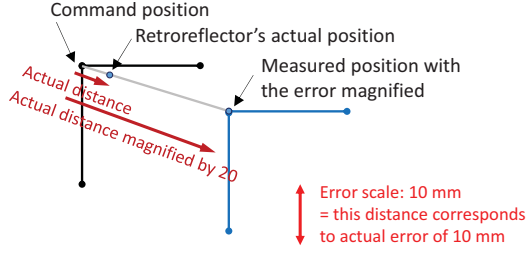
Fig. 11. The magnification of the error in the measured retroreflector position from its command position in Fig. 10.
