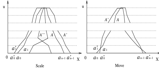
Figure 3: Scale and move transformations
