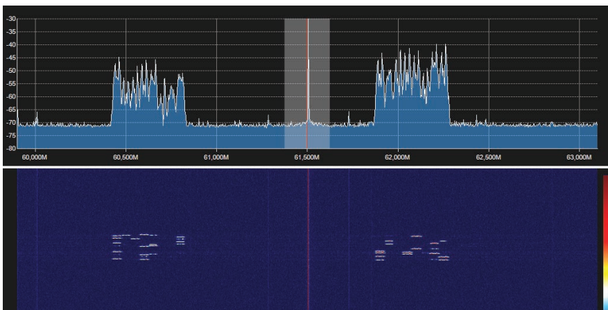
Fig 8. Simulation of the RCD and WF device under the influence of noise interference with frequency shift keying
