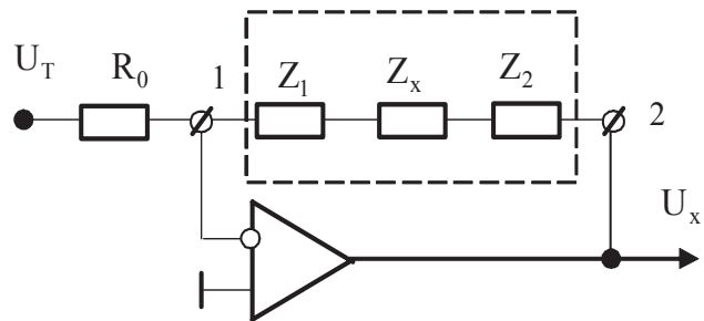
Fig. 2. Transducer of two-electrode sensor parameters with mode of given current
