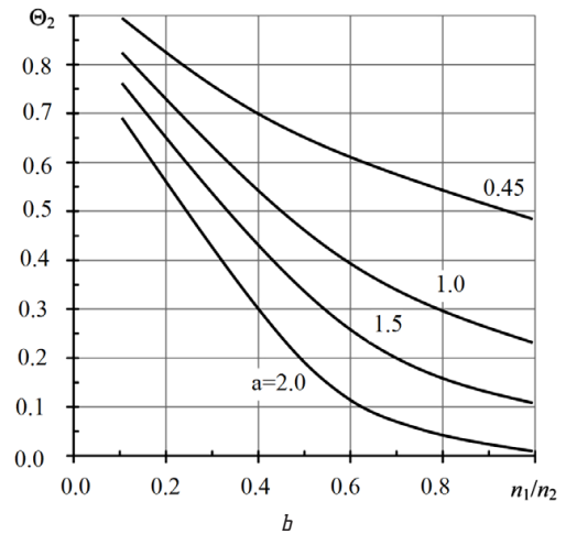
Fig. 3. Dependence of the temperature drop difference of cascades (stages) of a two-stage thermoelectric cooler on the ratio n_1/n_2 for different values of the parameter a at T=300 K; (I/S)_2=10 cm ^{-1} ; n_2=27 in the \Delta T_{\max} mode: a – the first stage \Theta_1 ; b – the second stage \Theta_2
