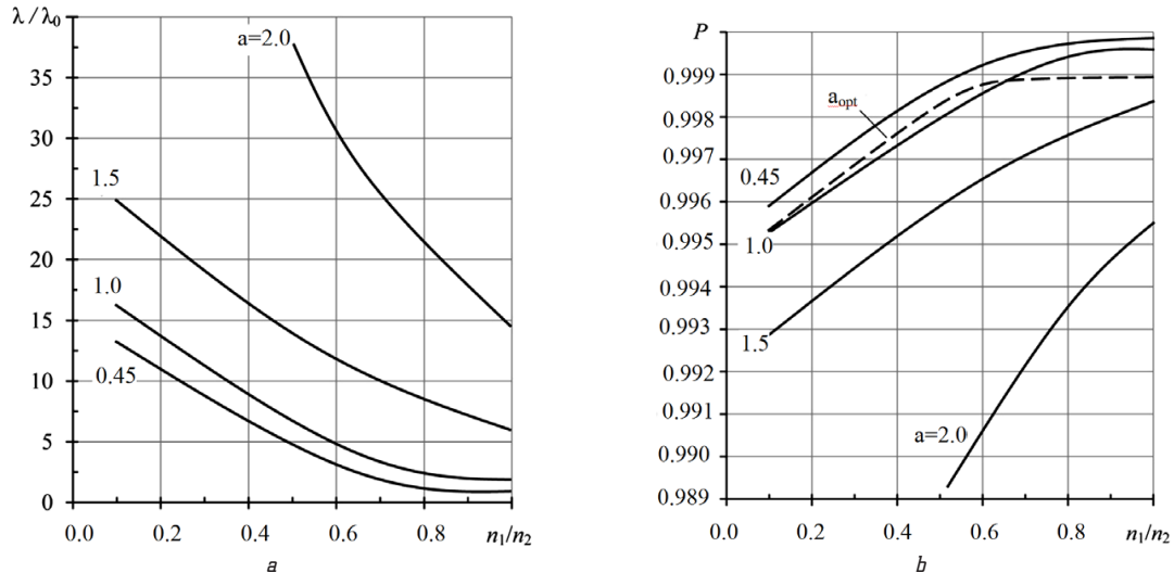
Fig. 6. Dependence of the relative failure rate \lambda/\lambda_0 and the probability of failure-free operation P of a two-stage thermoelectric cooling device on the ratio n_1/n_2 for different values of the parameter a at T=300 K; (l/S)_2=10 cm -1 ; n_2=27 in the \Delta T_{max} mode: a – relative failure \lambda/\lambda_0 ; b – probability of failure-free operation P
