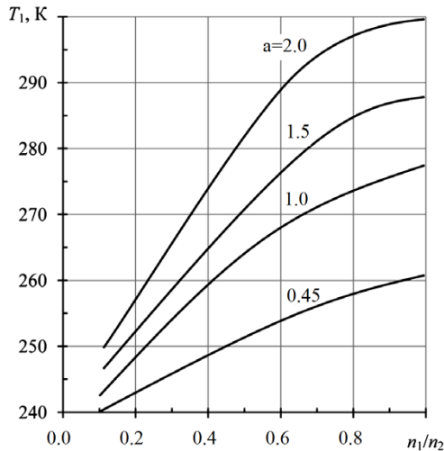
Fig. 1. Dependence of the intermediate temperature T_1 of a two-stage thermoelectric cooler on the ratio n_1/n_2 for different values of the parameter a at T=300 K; (I/S)_2=10 cm ^{-1} ; n_2=27 in the \Delta T_{\max} mode
