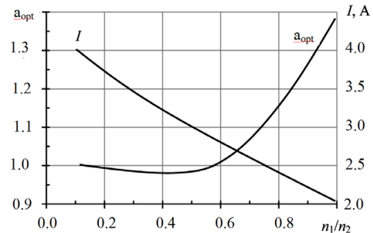
Fig. 4. Dependence of the optimum value of the parameter a corresponding to the largest value of the temperature drop: the vertex geometry parameter a and the working current I of the two-stage thermoelectric cooler on the ratio n_1/n_2 at T=300 K; (I/S)_2=10 cm ^{-1} ; n_2=27 in the \Delta T_{\max} mode
