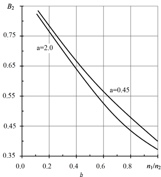
Fig. 2. Dependence of the relative operating current of cascades (stages) of a two-stage thermoelectric cooler on the ratio n_1/n_2 for different values of the parameter a at T=300 K; (I/S)_2=10 cm ^{-1} ; n_2=27 in the \Delta T_{\max} mode: a – the first stage B_1 ; b – the second stage B_2
