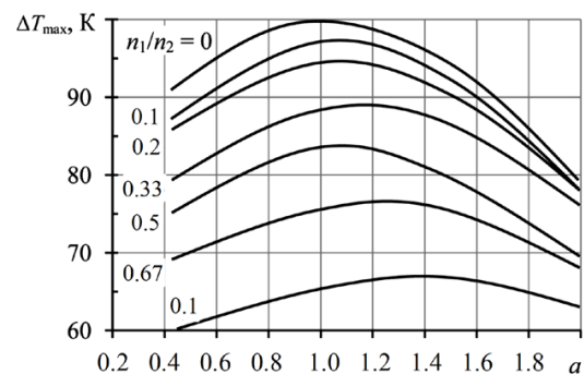
Fig. 5. Dependence of the maximum temperature difference \Delta T_{\max} of a two-stage thermoelectric cooler on the parameter a for different values of the ratio n_1/n_2 at T=300 K; (I/S)_2=10 cm ^{-1} ; n_2=27 in the \Delta T_{\max} mode
