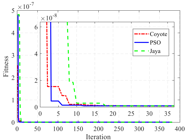
FIGURE 4. Convergence curves of the objective function for transformer; Case 1 (4 kVA, 380/380 V).
