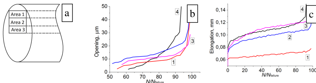
Figure 3. a) scheme of the rod and locations for cutting out specimens; b) crack opening graph; c) elongation during cyclic loading; 1) after the HR, area 1; 2) area 2; 3) area 3; 4) as-received state.
