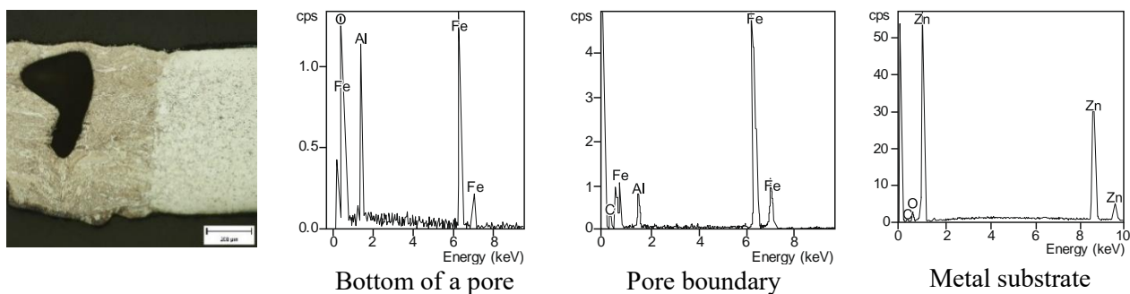
Figure 5. Micrograph of a pore and data of the EDX analyses.
