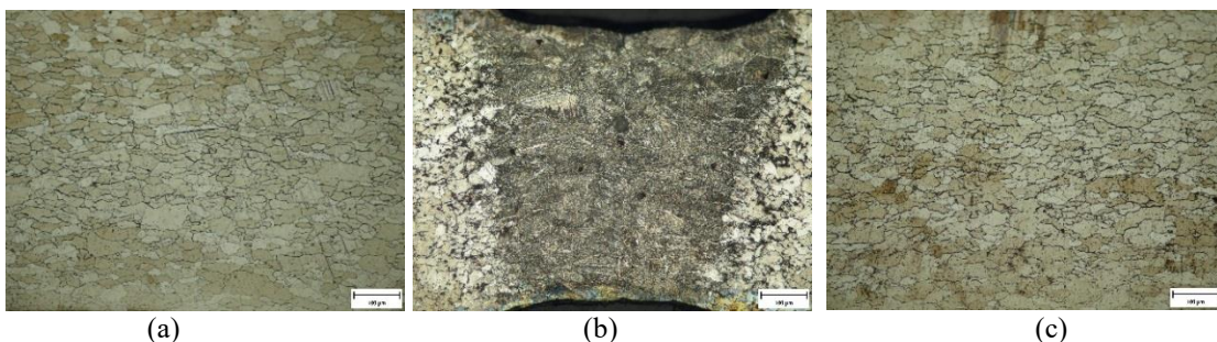
Figure 4. Structure of welded joint TWB2: a - base material DX53D+Z; b - weld and HAZ; c - base material DX54D+Z.
