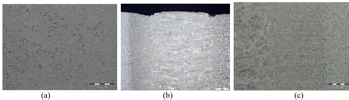
Figure 3. Structure of welded joint TWB1: a - base metal DX53D+Z; b – weld; c – HAZ 2 DX54D+Z.
