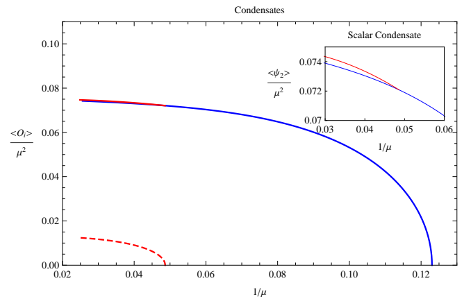
Figure 1: Condensates \psi^{(2)} (solid) and w^{(1)} (dashed) as a function of 1/\mu in the s -wave (blue) and s+p -wave (red) phases. The p condensate appears at \mu_{sp} such that \mu_s/\mu_{sp} = 0.395 as found in [20]. The inset zooms in on the plot of \psi^{(2)} to show the difference in the scalar condensate between the s (blue) and the s+p (red) solutions.
