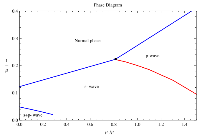
Figure 3: Phase diagram of the unbalanced system as a function of 1/\mu and \mu_3/\mu . Second order phase transitions are denoted by blue lines, whereas the red line corresponds to a first order phase transition.
