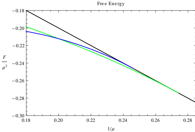
Figure 4: Free energy as a function of 1/\mu for \mu_3/\mu = -1 . Black corresponds to the normal phase, blue to the s -wave phase, and green to the p -wave phase.
