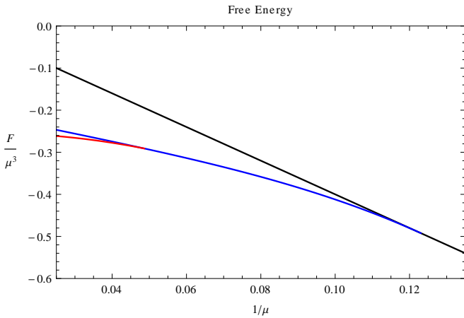
Figure 2: Free energy of the different solutions versus 1/\mu : normal phase in black, s -wave phase in blue, and s+p -wave phase in red.
