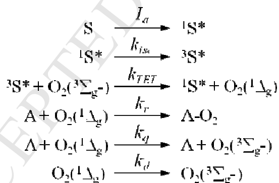
Scheme 2. Simplified mechanism for photosensitized ADPA oxidation.
