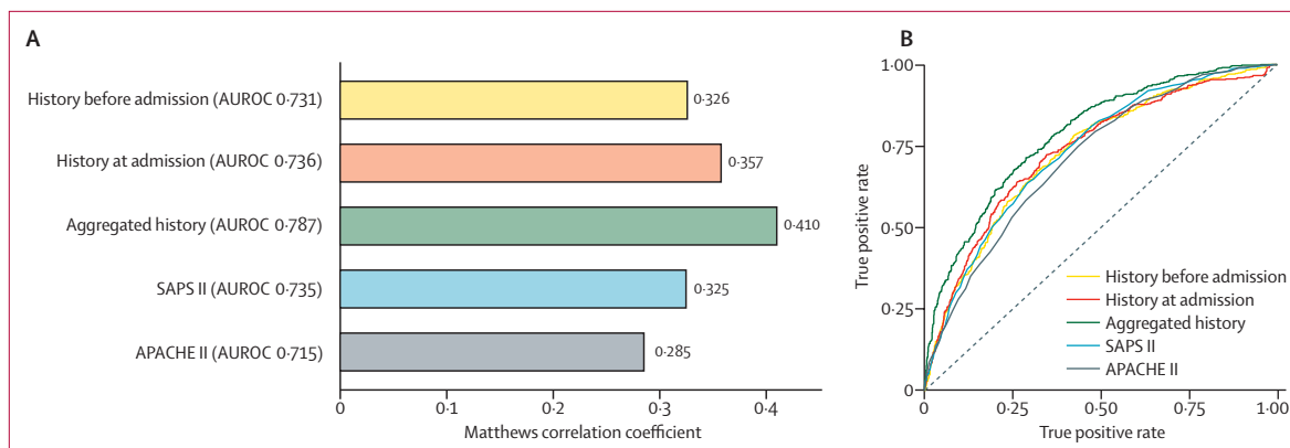
Figure 3: Matthews correlation coefficients (A) and AUROC (B) for models with input data from different timepoints 90-day mortality was the outcome measure for this figure. The history before admission model was trained on age, sex, and 10-year disease history before ICU admission. The history at admission model also included transfer category (ie, medical, scheduled surgery, or unscheduled surgery), length of stay before ICU admission, and hospital code. The aggregated history model included an aggregated dataset with both long-term disease history (ie, the data used in the history at admission model) and data for the first 24 h of ICU admission (ie, features included in SAPS II and APACHE II combined). In these three models, disease history was presented as an accumulated representation because the cohort was too small for year-wise representation (appendix). In figure 3B, the dotted line represents the AUROC of a model with a random guess. AUROC=area under the receiver operating characteristic curve. ICU=intensive-care unit. SAPS II=Simplified Acute Physiology Score II. APACHE II=Acute Physiologic Assessment and Chronic Health Evaluation II.
