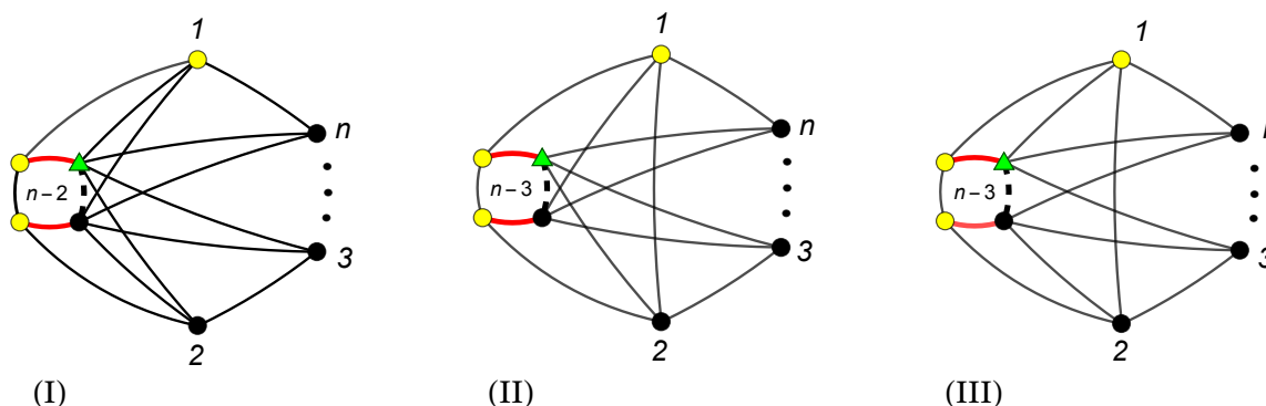
Figure 5. Simplest cases of CHY-graphs from figure 4.
