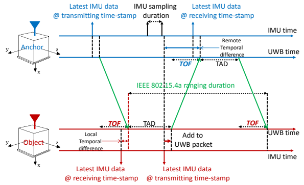
Fig. 2: Fully-coupled data communication and synchronization.
