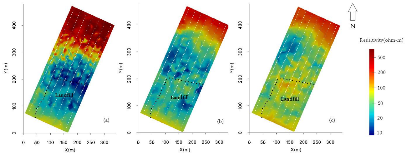
Figure 6 3D DC inversion result shown as horizontal resistivity map at different elevation. (a)-30m, (b)-20m, (c)-10m, Boundary of the landfill is shown by black dotted line and position of the electrodes is shown as white dots.
