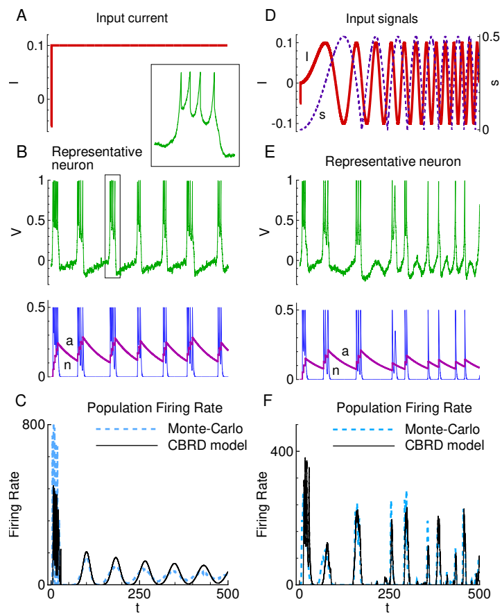
Fig. 5 Population of bursting neurons with potassium current. A-C : Response to a step of current. D-F : Response to a complex-shaped current. A,D : Input current I(t) and conductance s(t) . B,E : Membrane voltage of a single neuron. The green traces are the voltage responses, while the time trajectory of the recovery variable, a and the potassium gating variable n are shown in purple and blue, correspondingly. C,F : Population firing rate, calculated in Monte-Carlo simulation and the CBRD model. 20000 trials were used in the Monte-Carlo simulations.
