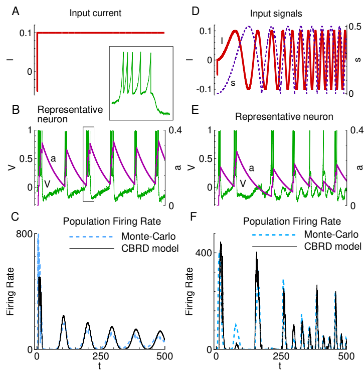
Fig. 3 Population of bursting neurons. A-C : Response to a step of current. D-F : Response to a complex-shaped current. A, D : Input current I(t) and conductance s(t) . B, E : Membrane voltage of a single neuron. The green traces are the voltage responses, while the time trajectory of the recovery variable, a is shown in purple. C, F : Population firing rate, calculated in Monte-Carlo simulation and the CBRD model. 20000 trials were used in the Monte-Carlo simulations.
