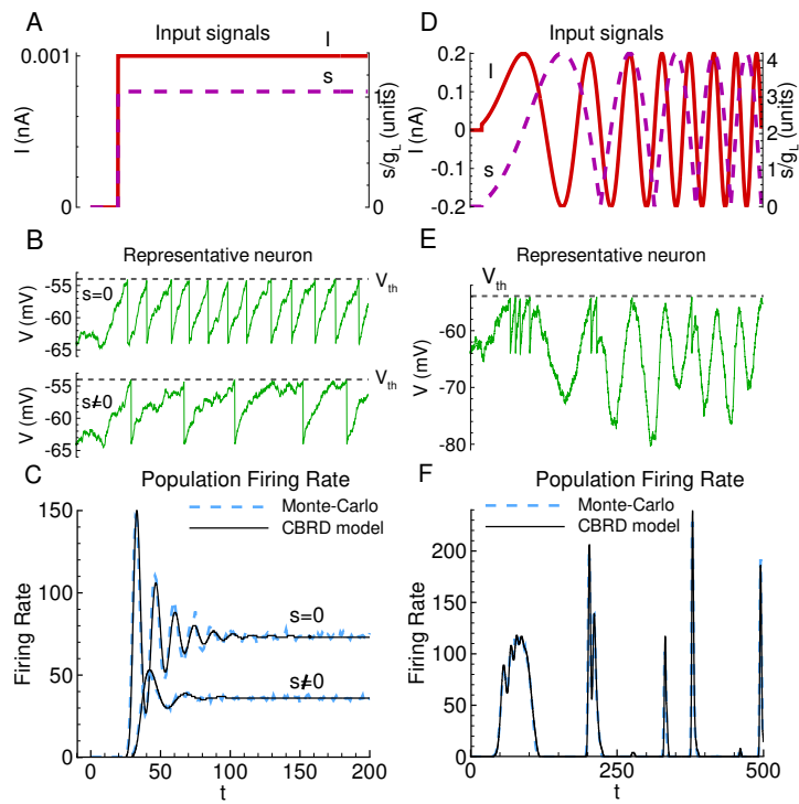
Fig. 2 Population of LIF neurons. A-C: Response to step-wise stimuli. D-F: Response to a complex-shaped current. A,D: Input current I(t) and conductance s(t) . B,E: Membrane voltage of a single neuron. C,F: Population firing rate, calculated in Monte-Carlo simulation and the CBRD model. 50000 trials were used in the Monte-Carlo simulations.
