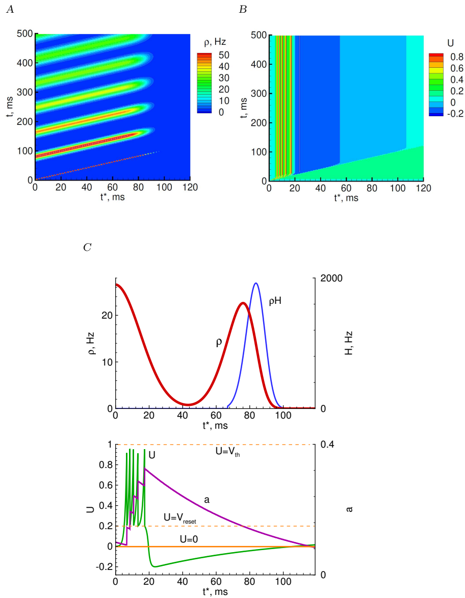
Fig. 4 This plot extends Fig. 3A-C. Specifically, it depicts t^* - t -plots for the neuronal density \rho (A) and voltage U (B), that lead to the firing rate response shown in Fig. 3C. Panel C shows the profiles in t^* -space at t = 500 ms for the neuronal density \rho and the source term \rho H (middle panel), and the mean voltage U and adaptation a (bottom panel).
