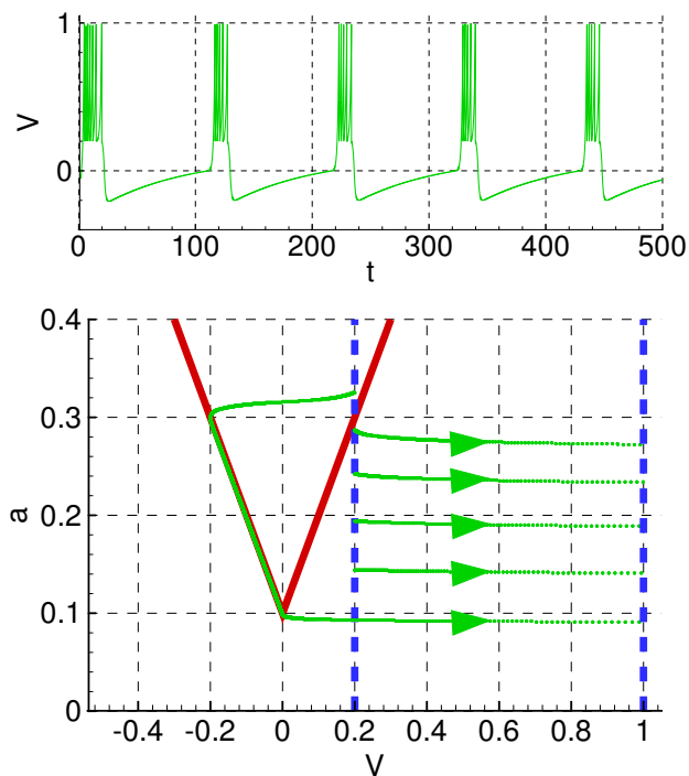
Fig. 1 Hybrid model for bursting neuron. Voltage trace (top) and phase-space plot (bottom) with nullclines (red and blue) and a trajectory (green). The red nullclines intersect at hyperplane V = 0 , which corresponds to the true neurophysiological threshold (seen from the perspective of smooth continuous time slow-fast systems). The dashed blue line (left) correspond to the V_{reset} and the dashed blue line (right) correspond to V_{th} .
