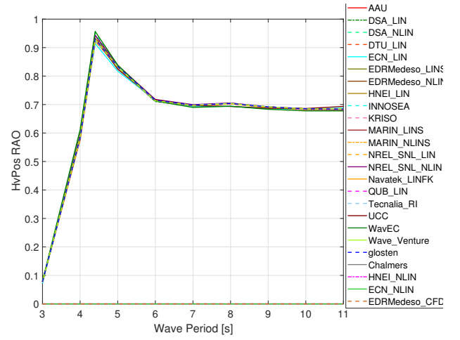
Fig. 6. Heave RAO, optimum PTO damping, S=0.002 .
