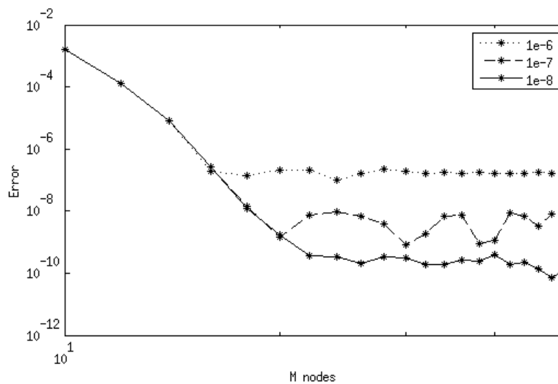
Figure 3.15: Error of the rightmost eigenvalue with respect to the number M of Chebyshev extremal nodes for different relative tolerances R_{tol} of the DOPRI5 method.
