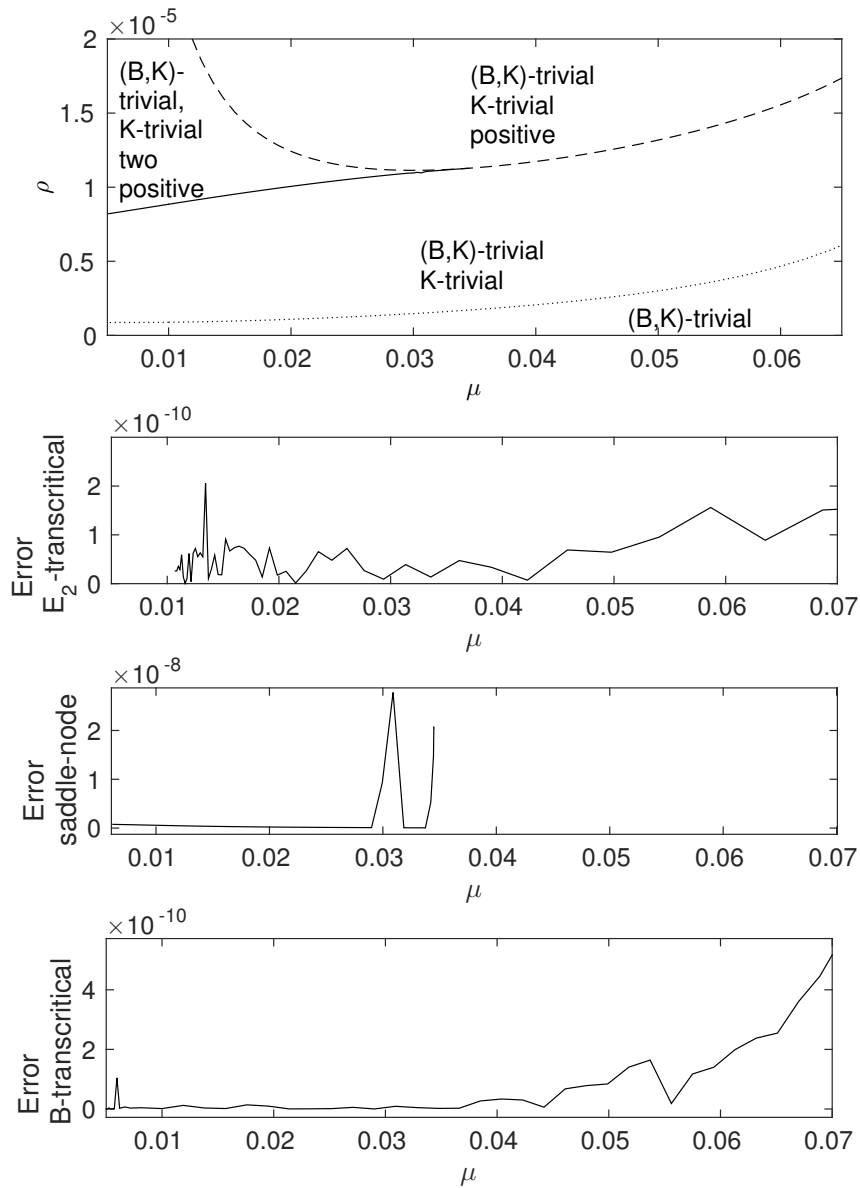
Figure 4.8: (\mu, \rho) -parameter plane and regions of existence of equilibria (upper panel). B -transcritical (dotted), E_2 -transcritical (dashed), and saddle-node (continuous) bifurcations for the three trophic model. Errors (rest of the panels) for a maximum step size of 0.002 for the tangent prediction and a tolerance of 10^{-7} for the Quasi-Newton method.
