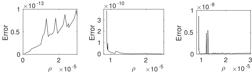
Figure 4.6: Errors of the \mathcal{K} -trivial equilibrium branch (left panel) and of the positive branches (center and right panels) in Figures 4.4 and 4.5 for a maximum step size of 1.5 \times 10^{-6} and a tolerance of 10^{-8} for the Quasi-Newton method.
