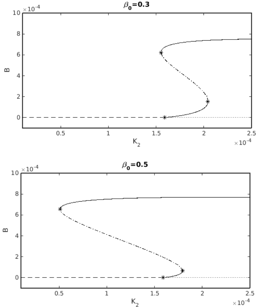
Figure 4.15: Detail of Figure 4.14 for \beta_0 = 0.3 and \beta_0 = 0.5 .
