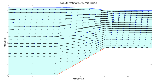
(b) Velocity vector
