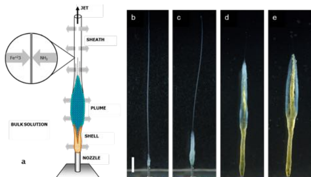
Figure 8: Precipitation templated by a fluid jet. (a) Schematic representation of the stages of growth around a jet of aqueous ammonia injected into an iron sulfate solution, and the subsequent oxidation of the precipitate. (b) 1 min after start, (c) 5 min, (d) 45 min, and (e) 125 min. Scale bar is 5 mm. Reprinted with permission from ref 43. Copyright 2005 American Chemical Society.
