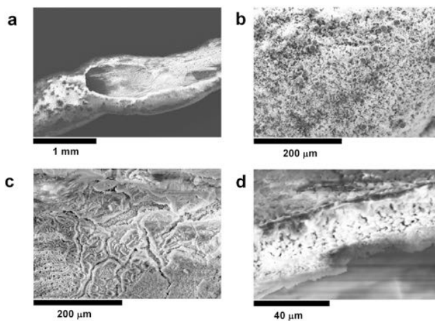
Figure 19: SEM images of (a) single fracturing precipitation tube, (b) exterior surface, (c) interior surface and (d) tube wall. Adapted with permission from ref 124. Copyright 2011 Elsevier.
