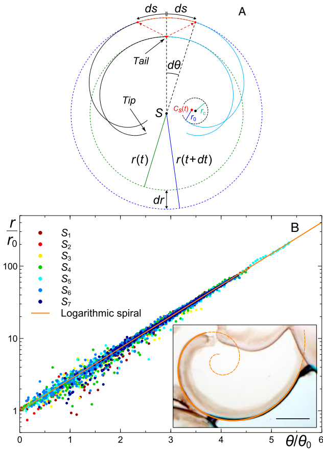
Figure 29: Spiral growth mechanism and scaling of logarithmic spiral-shaped precipitates. (a) Schematic of the growth mechanism of the curly shaped precipitates during an infinitesimal interval of time where r(t) is the radius of the expanding bubble of injected reagent and S is the point source. (b) Scaling law for the experimentally measured evolution of the radial distance r/r_0 as a function of the scaled angle \theta/\theta_0 for 173 spirals (9 experiments). (Inset) Superimposition of a logarithmic spiral on a spiraled precipitate. (Scale bar, 2 mm.) Reprinted with permission from ref 38. Copyright 2014 Haudin et al.
