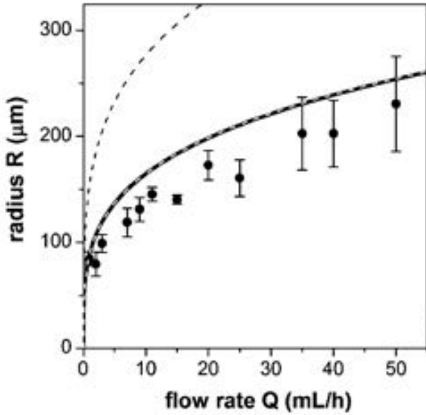
Figure 26: Jetting data are shown along with the solutions of purely hydrodynamic equations. The lower curve corresponds to a model specified in Eq. (4). The upper dashed curve corresponds to the stiff tube model, i.e., Eq. (4) for \eta_o \rightarrow \infty . Reprinted with permission from ref 41. Copyright 2004 European Physical Society.
