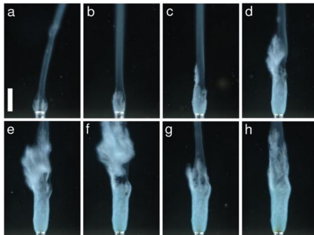
Figure 30: Close-up of a growing tube. The sequence of images spans 5 minutes with panels d–g taken 15 seconds apart. Tube growth begins in (a) as precipitate attached to nozzle, followed by transient elongation (b–d), detachment of a section (e, f), and finally, regrowth (g, h). Scale bar is 2 mm. Reprinted with permission from ref 43. Copyright 2005 American Chemical Society.
