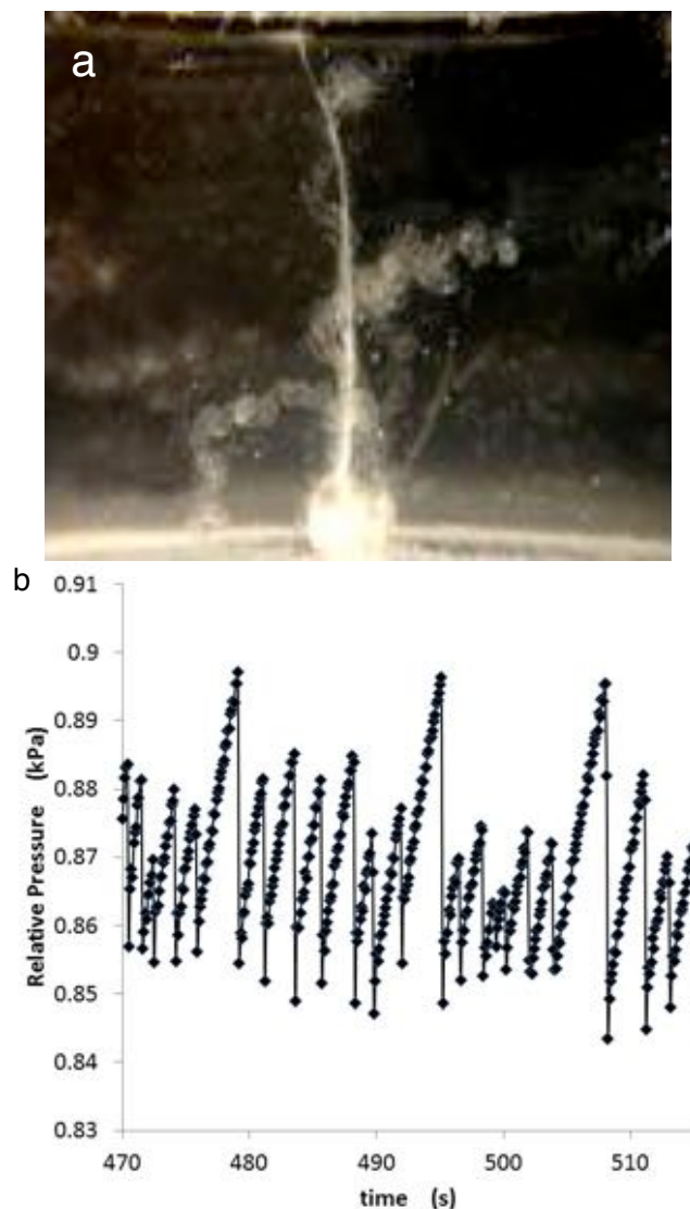
Figure 24: (a) An example of a moving structure with three “arms”. The two horizontal arms move up and down in synchronized motion. The pellet at the bottom of the structure has a diameter of 1 cm. 122 (b) Changes of pressure inside the moving structure as a function of time. 123 Reprinted with permission from refs 122,123. Copyright 2008, 2009 American Physical Society.
