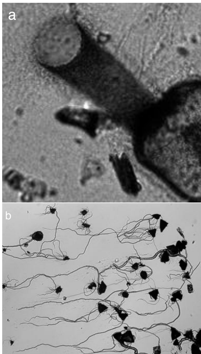
Figure 39: (a) A microtube approximately 50\ \mu\text{m} in diameter growing on a glass surface. (\text{C}_4\text{H}_{10}\text{NO})_{40}[\text{W}_{72}\text{Mn}_{12}\text{O}_{268}\text{Si}_7] \cdot 48\text{H}_2\text{O} POM in N-methyl dihydroimidazolphenanthridinium bromide solution. Image from Geoff Cooper. (b) Several microtubes approximately 25\text{--}75\ \mu\text{m} in diameter under bulk flow conditions, showing the alignment of the growth direction to the flow. Reprinted with permission from ref 115. Copyright 2011 American Chemical Society.
