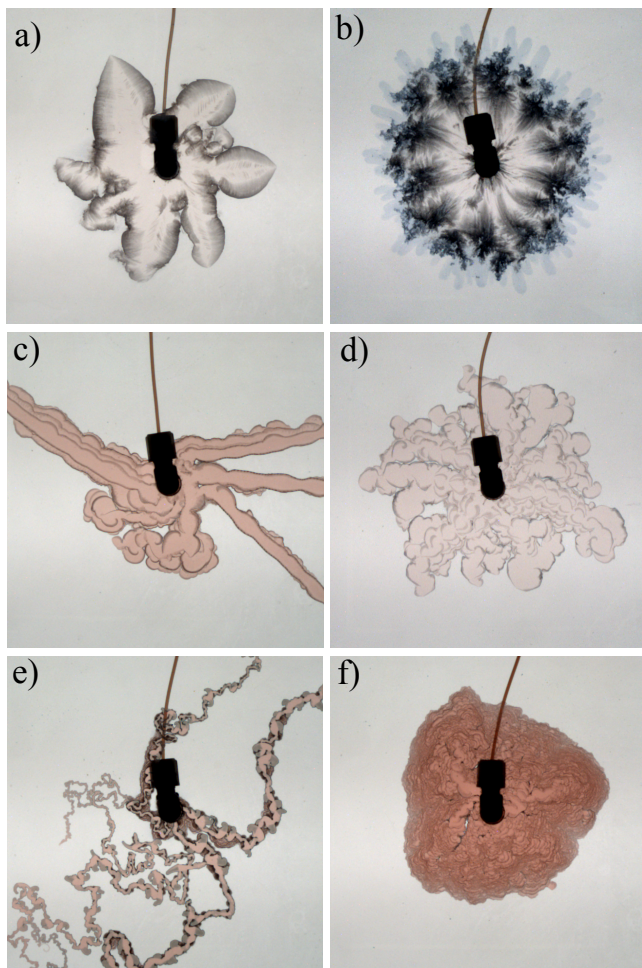
Figure 15: 2D chemical gardens: Patterns obtained after t = 30 s for cobalt chloride injected into sodium silicate in a Hele-Shaw cell for various concentrations at a fixed flow rate. The field of view is 15 \times 15 cm. Adapted in part with permission from ref 38. Copyright 2014 Haudin et al.
