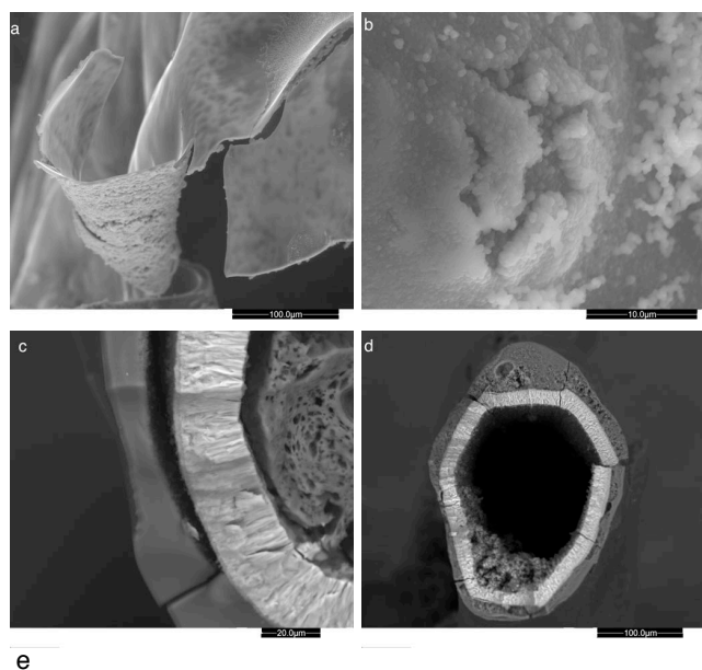
Figure 19: SEM images of (a) single fracturing precipitation tube, (b) exterior surface, (c) interior surface and (d) tube wall. Adapted with permission from ref 124. Copyright 2011 Elsevier.
