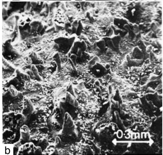
Figure 35: (a) Nodule of \text{Fe}_3\text{O}_4 and green rust showing vent which formed on grey cast iron in water at 50^\circ\text{C} and 0.44 \text{ ppm O}_2 after 7 h. (SEM). (b) Open-topped 'chimneys' growing out of crusted scale formed after 25 h on grey cast iron in water at 50^\circ\text{C} and 3.00 \text{ ppm O}_2 . (SEM, 60^\circ tilt). Reprinted with permission from ref 175. Copyright 1979 Elsevier.
