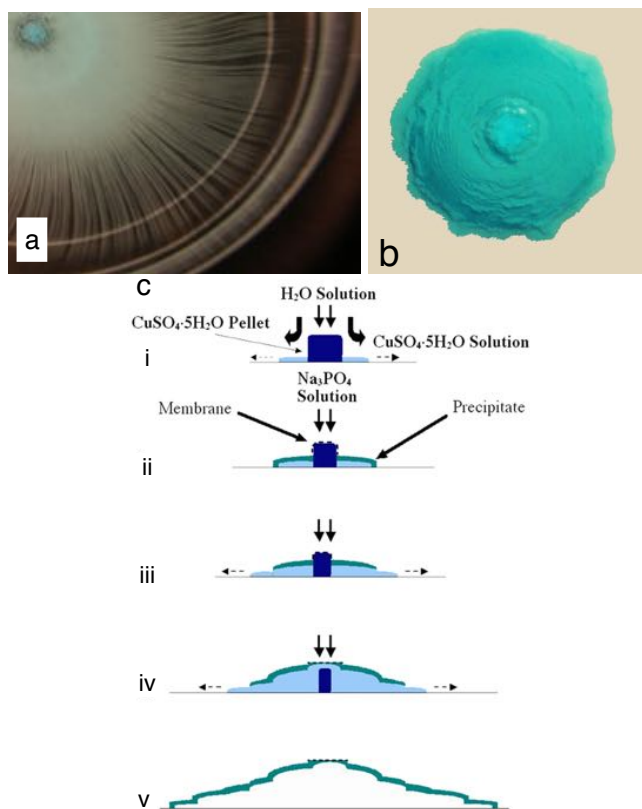
Figure 16: (a) Horizontal structure in the \text{Cu}^{2+} -oxalate system; 96 the initial pellet is visible. The structure is about 10 cm in diameter. (b) The structure that grows on the bottom of the experimental dish in the \text{Cu}^{2+} -phosphate system. 97 The structure forms a dome with successive layers visible. The structure is about 10 cm in diameter. (c) Sketch of growth dynamics of copper-phosphate structure. 96 (i, ii) The copper pellet dissolves forming a solution with greater density. This solution flows to the bottom under gravity and spreads out. On the top of the solution the membrane/precipitate is growing. It stops spreading of the solution. (iii) Osmotic pressure forces water inside the membrane, lifting a layer of the structure up. (iv, v) The solution spreads, further membrane is formed and the process repeats. Reprinted with permission from refs 96,97. Copyright 2009, 2003 American Chemical Society, Elsevier.
