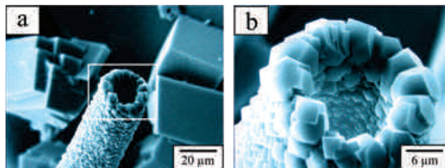
Figure 11: (a) SEM image of a tubular aggregate of calcium carbonate formed on a cation-exchange membrane. (b) The magnified image of the rectangular area in panel a. Reprinted with permission from ref 60. Copyright 2006 American Chemical Society.
