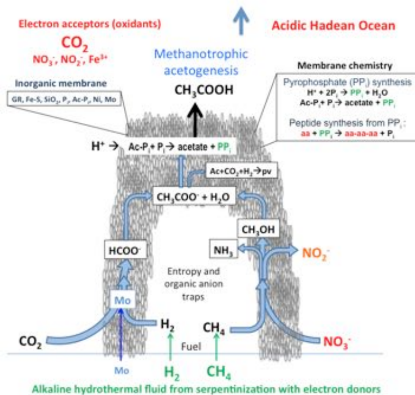
Figure 43: A natural compartmentalized chemical garden (hydrothermal mound) over an alkaline vent (exhaling sulfide containing solution) in the ancient Hadean carbonic ocean (anoxic and therefore enriched in dissolved \text{Fe}^{2+} ). 49 The chemiosmotic potential is derived from the partial dissolution of the olivine and minor pyruvate comprising komatiite, peridotite, or harzburgite beneath the hydrothermal mound (not shown) to produce an alkaline hydrothermal fluid, against the acidic (carbonic) ocean. Interaction between the two fluids in the green rust (GR)-bearing membrane could have driven the synthesis of formate ( \text{HCOO}^- ), acetate (ac, \text{CH}_3\text{COO}^- ), pyruvate (pv), and thereby, amino acids (aa) and peptides (aa-aa-aa) 220–222 while the chemiosmotic potential may have driven pyrophosphate ( \text{PP}_i ) formation from orthophosphates ( \text{P}_i ) and acetyl phosphate (Ac-Pi). Redrawn with permission from ref 207. Copyright 2013 the Royal Society.
