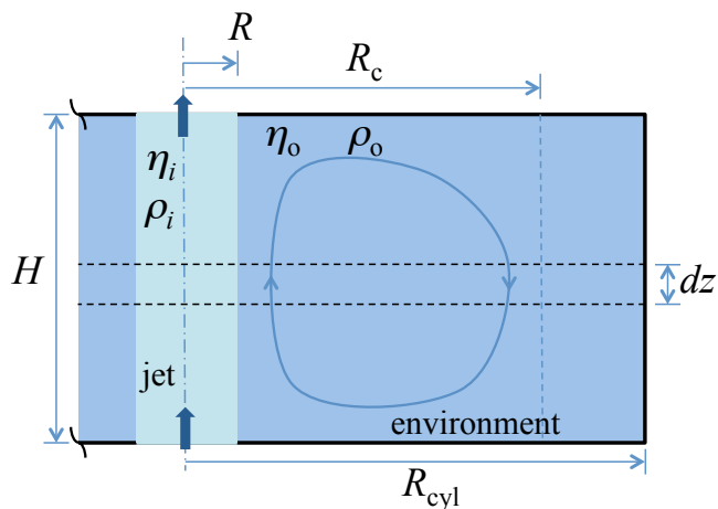
Figure 25: Sketch of the model setup with a fluid jet and recirculation of the fluid in the environment around it, that leads to Eqs 2, 4, and, with \eta_o \rightarrow \infty , to Eq. 5.
