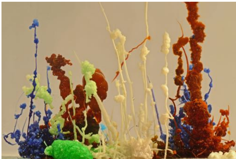
Figure 1: A classical chemical garden formed by the addition of cobalt, copper, iron, nickel, and zinc salts to a sodium silicate solution. The image corresponds to 5.5 \times 3.7 cm. Image courtesy of Bruno Batista.
