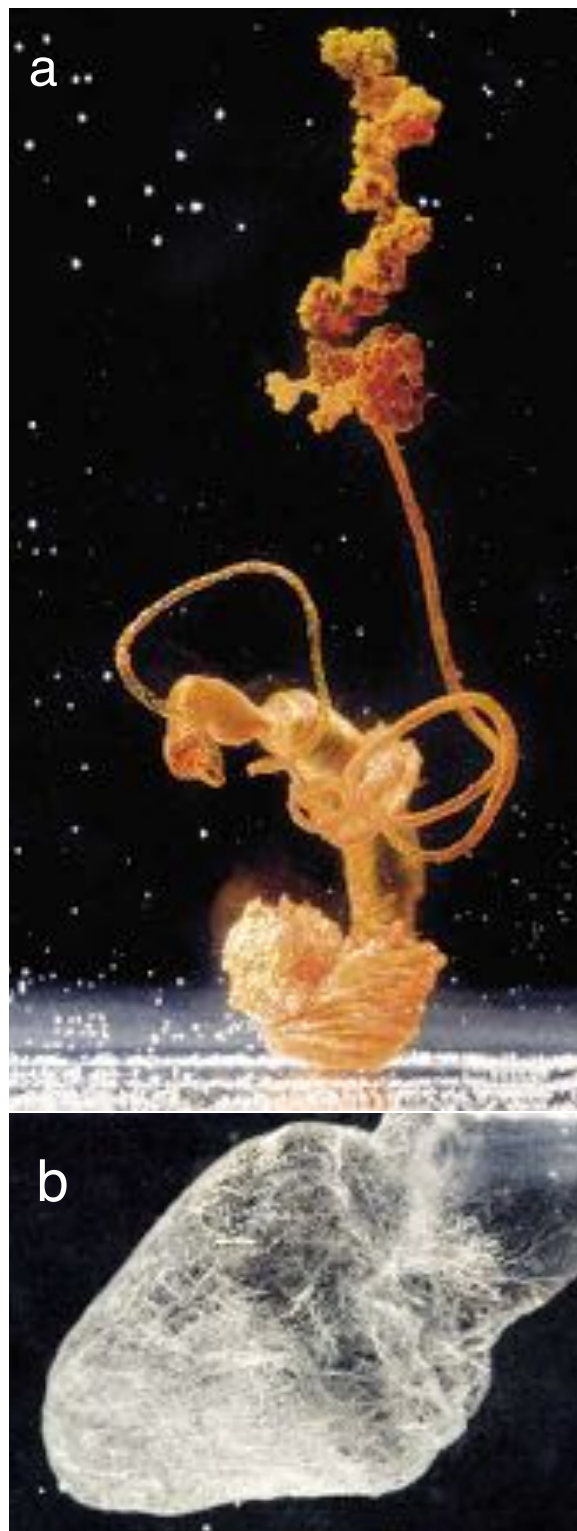
Figure 4: Two examples of Eastes and Darrigan's modern recreations of Leduc's work. (a) Sodium silicate solution with an iron(III) chloride seed. (b) Sodium carbonate and sodium phosphate solution with a calcium chloride seed. Reprinted with permission from ref 20. Copyright 2006 xxx.
