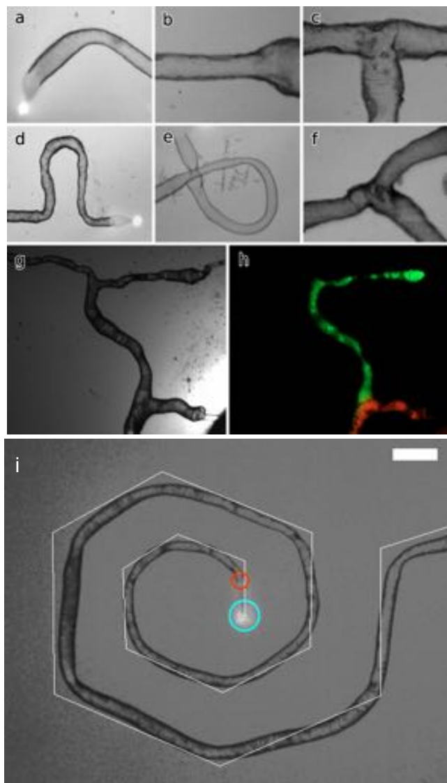
Figure 40: A laser control system can produce devices using a number of basic elements: (a) a wide bend, (b) a change in diameter, (c) a ‘T’ junction produced by puncturing a growing tube, (d) a sharp bend, (e) tubes crossing, (f) a ‘Y’ junction produced by merging two tubes, (g) a device comprised of two ‘Y’ junctions between three individual tubes and (h) the same device with green (Fluorescein) and red (Rhodamine B) fluorescent dyes flowing into the junctions. Tubes are between 20–50 \mu\text{m} in diameter. (i) Automated control of a laser spot to grow a tube to a specified pattern (a spiral). The blue marker shows the laser spot position, the red marker shows the position of the growing tube (by image analysis) and the white line shows the pre-loaded pattern. Scale bar is 500 \mu\text{m} . Images from Geoff Cooper.
