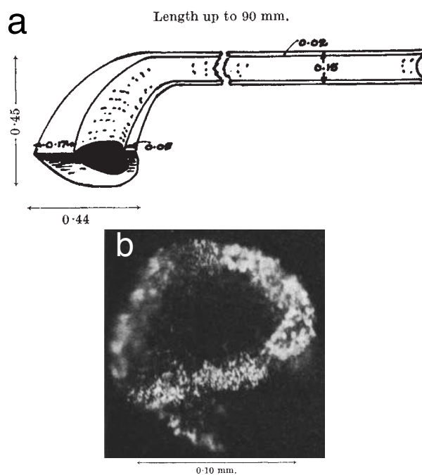
Figure 33: (a) Sketched longitudinal section and (b) micrograph cross section of tubular forms of iron rust. Reprinted with permission from ref 171. Copyright 1958 Macmillan Publishers Ltd.
