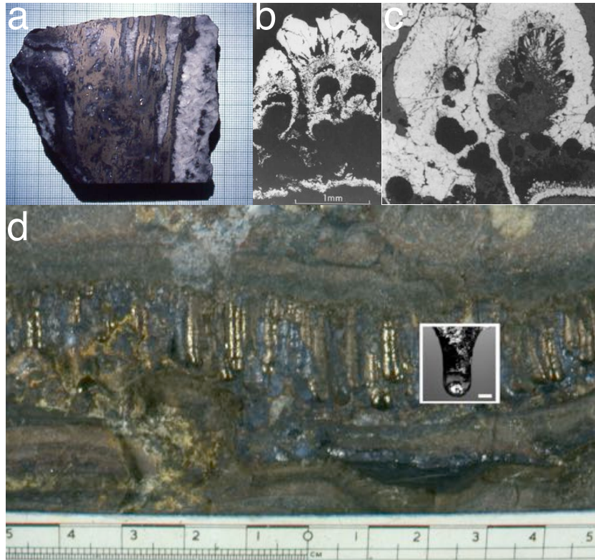
Figure 42: (a) A natural iron sulfide garden from the Tynagh mine, Ireland, now composed of pyrite embedded in barite, produced as a somewhat acidic, iron(III)-bearing buoyant hydrothermal solution invaded a mildly alkaline sulfanide (bisulfide)-bearing brine occupying a void below the Carboniferous seafloor \sim 350 million years ago (Russell and Hall 140 , cf., jetting, Section 3.2); (b, c) hollow pyrite botryoids produced as for (a) but perhaps more slowly (Russell and Hall 140 , cf., budding, Section 3.2); (d) reverse gardens found at Navan, also in Ireland, whereby a dense sulfanide-bearing surface brine seeped down into an open horizontal joint occupied by iron-bearing mineralizing solution \sim 350 million years ago. 205 A photograph of a comparable reversed-phase growth of a “hanging” iron(III) sulfide budding tube produced as iron(III) sulfate was passed down into gaseous H_2S is superimposed on the geological sample (cf. Stone and Goldstein 44 , fig. 6 and the reverse chemical gardens of Pagano et al. 47 , Section 3.1). Adapted with permission from ref 140. Copyright 2006 GSA.
