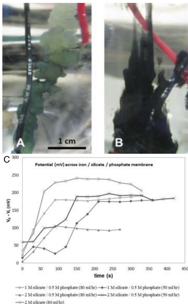
Figure 20: Chemical-garden structures grown via injection of (a) acidic \text{FeCl}_2 solution into alkaline silicate solution; and (b) alkaline sodium sulfide/silicate solution into acidic \text{FeCl}_2 -containing solution. A wire was placed near the injection point so that the membrane would envelop the wire as it grew, while a second wire was placed in the outer solution. A membrane potential is generated immediately upon precipitation, and the value of the membrane potential is characteristic of the reactant system and concentrations chosen. (c) Shows potentials generated by Fe(II)–silicate–phosphate chemical gardens formed with varying reactant concentrations and injection rates. (a,b) Images from Laurie Barge; (c) Reprinted with permission from ref 37. Copyright 2012 American Chemical Society.
