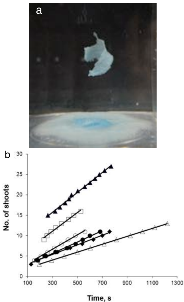
Figure 23: (a) A pellet of copper chloride in a solution of sodium carbonate leads to the formation of a precipitate structure that is periodically ejected from the pellet. The period is about 1 minute and the process may continue for an hour. The width of the image corresponds to 5 cm. (b) The number of membrane pieces that have been ejected as a function of time for various carbonate concentrations. The [\text{CO}_3^{2-}] molarity is: black triangles, 0.16 M, open squares, 0.13 M, open circles, 0.11 M, black circles, 0.09 M, black diamonds, 0.07 M, open triangles, 0.06 M. Note that the data are linear and the slope is increasing with the concentration of carbonate. Reprinted with permission from ref 107. Copyright 2005 Springer Science and Business Media.
