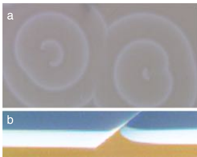
Figure 12: Traveling precipitation waves, including counterrotating spiral waves, are observed in the precipitation reaction of \text{AlCl}_3 with \text{NaOH} . (a) Image, taken from above, of waves in a gel disk within a Petri dish. (b) Image of a wave traveling in a gel containing the pH indicator bromothymol blue (with front illumination). Reprinted with permission from ref 86. Copyright 2013 American Chemical Society.
