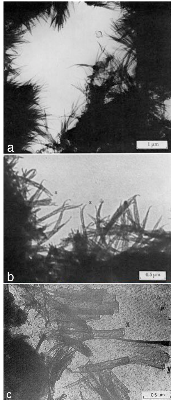
Figure 37: Cement tubes: (a) Cement + water sample after more than 1 day showing the secondary fibrillar development of C-S-H gel around the cement grains. (b) Greater detail of fibers. Environmental specimen stage, high voltage electron microscope. (c) Dried cement sample showing fibrillar C-S-H hydration product, the appearance of which suggests tubular morphologies. Transmission electron micrograph. Reprinted with permission from ref 177. Copyright 1976 Macmillan Publishers Ltd.
