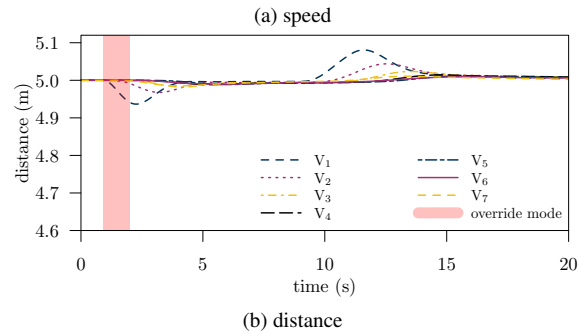
Figure 12: Dynamics of the platoon in response to a slower vehicle cut in maneuver, for a cut in distance of 50 m and a relative speed of 20 km/h.
