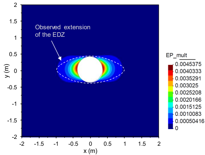
Figure 6: Obtained configuration of the EDZ in terms of plastic multiplier in the section a at the end of excavation.
