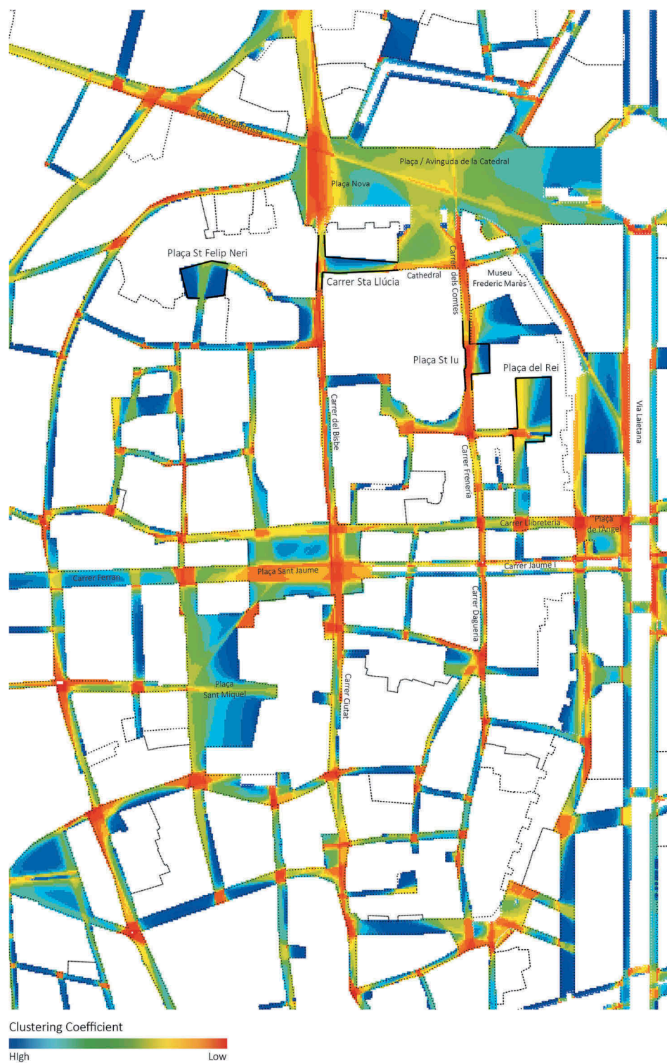
Figure 3. Clustering coefficient analysis of central Ciutat Vella, Barcelona. Within this framework the values range from 0.42 (red) to 0.98 (blue).
