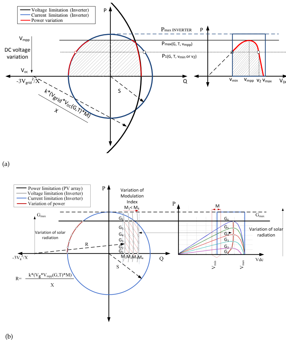
Figure 14. PQ capability curve of a PV generator (a) Variable dc voltage (b) Variable Modulation index [30] (Reproduced from Solar Energy, Vol 140, Ana Cabrera et al., “Capability curve analysis of photovoltaic generation systems”, Copyright (2016), with permission from Elsevier).
