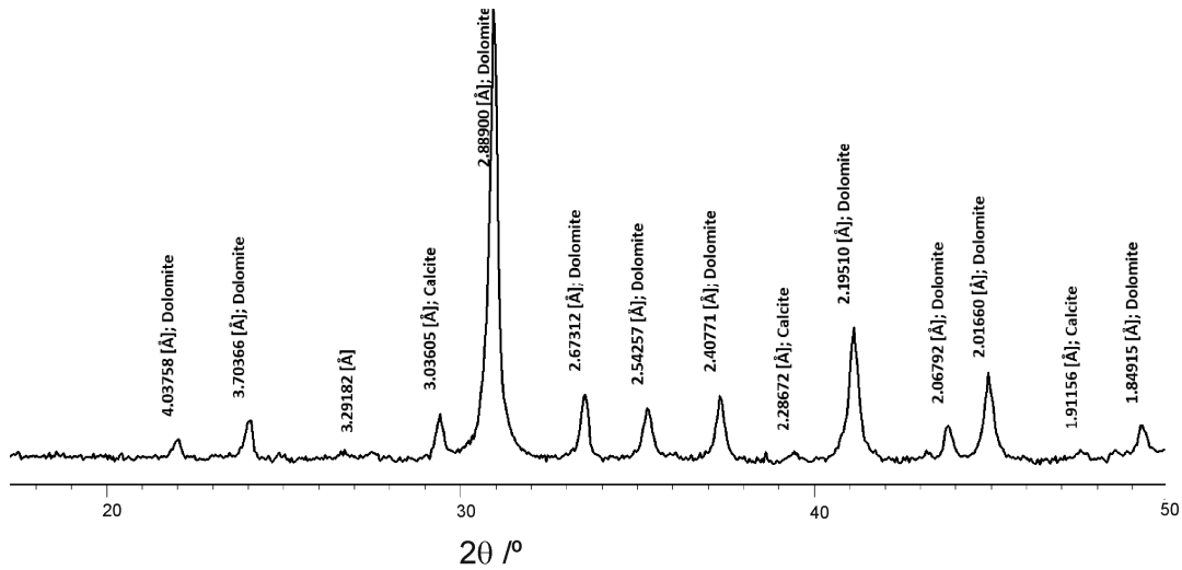
Figure 2. XRPD (x-ray powder diffraction) pattern of the dolostones used as aggregates to make the Camarasa concrete.
