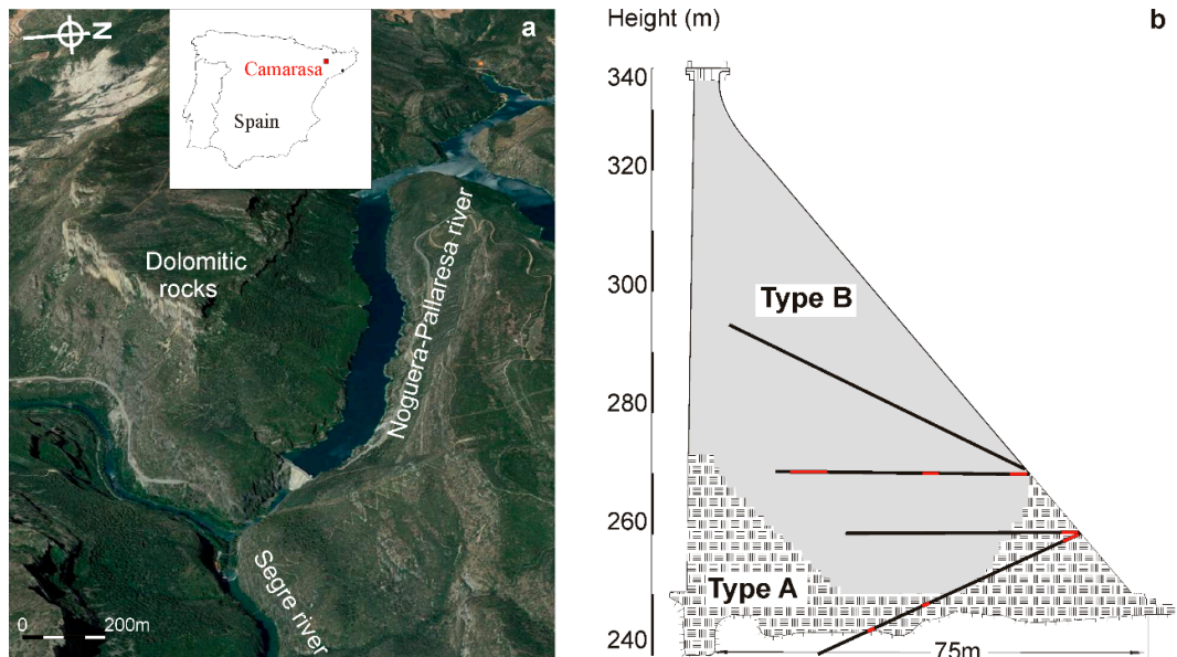
Figure 1. (a) View of the Camarasa Dam; (b), sketch with the distribution of the two concrete types (modified from [26] and the location of the cores (black lines) and samples (red)).
