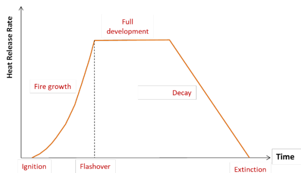
Figure 2. Example of a typical fire curve.
