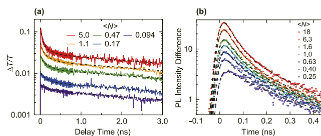
FIG. 4. (a) Excitation fluence dependence of the TA decay curves monitored at the CsPbBr 3 NC exciton ground state energy. The excitation fluence is expressed in terms of average absorbed photons per NC. The decay curves are fitted using triple exponential functions (dashed curves). (b) Fast decay components of the PL curves as a function of the excitation fluence. The resulting curves are fitted using double exponential functions. Figures are adapted with permission from Yarita et al. , J. Phys. Chem. Lett. 8 , 1413 (2017). Copyright 2017 American Chemical Society.
