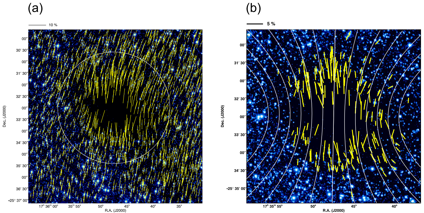
Figure 1. (a) Polarization vectors of point sources in FeSt 1-457 superimposed on the intensity image in the H band. The scale of the 10% polarization degree is shown above the image. (b) Polarization vectors of FeSt 1-457 after subtracting the ambient polarization component. The field of view is the same as the diameter of the core ( 288'' or 0.19 pc). The white lines indicate the magnetic field direction inferred from the fitting with a parabolic function. The scale of the 5% polarization degree is shown above the image. These figures are taken from Paper I.
