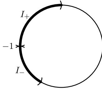
Figure 1: Intervals I_\pm .
