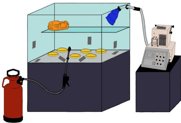
Figure 1: Representation of the experimental apparatus showing the chemical hood, the automatic atomizer (for the dispersion of S. cerevisiae ) and the HPV production system. The system is sealed and no hydrogen peroxide vapor is allowed to escape. Petri dishes (in yellow) were placed on the worktop of the hood together with the automatic air sampler (orange), to collect samples of S. cerevisiae . Stainless steel indicators (grey rectangles) inoculated with G. stearothermophilus were placed on the worktop and on the internal walls of the hood.
