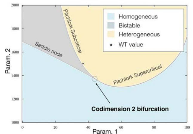
Fig. 2. Two-dimensional bifurcation diagram for two different parameters. The curves for the three types of bifurcations divide the parameter space into different phenotypes of our two-cell system: heterogeneous in yellow, bistable in grey and homogeneous in blue. The wild-type value for the pair of parameters is represented as an asterisk.
