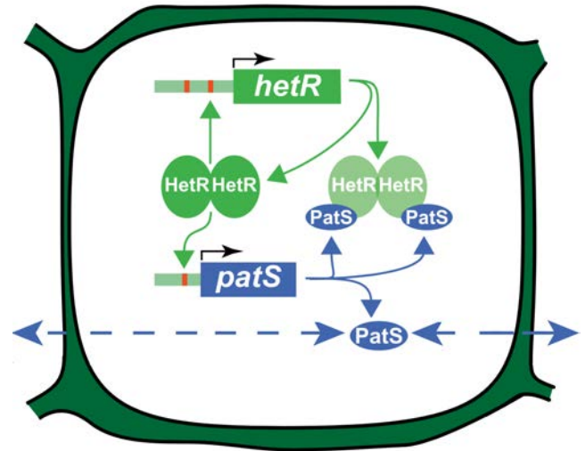
Fig. 1. Minimal model of the genetic network involved in heterocyst pattern formation at early stages. This network includes mechanisms of local autoactivation via HetR dimers and long-range inhibition governed by PatS, that is able to bind and inhibit HetR dimers and also to diffuse between cells (blue dashed arrows).
