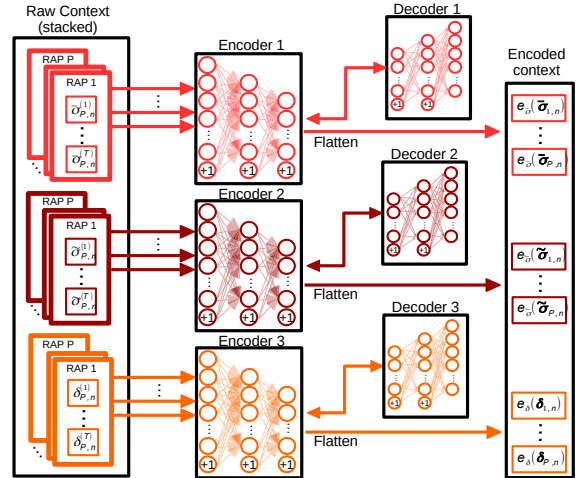
Figure 7: Encoder design.
