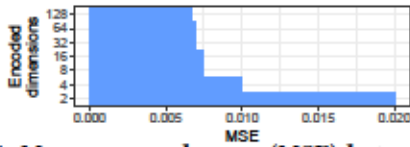
Figure 11: Mean squared error (MSE) between validation dataset and reconstructed sequences after encoding for a variable number of latent dimensions.
