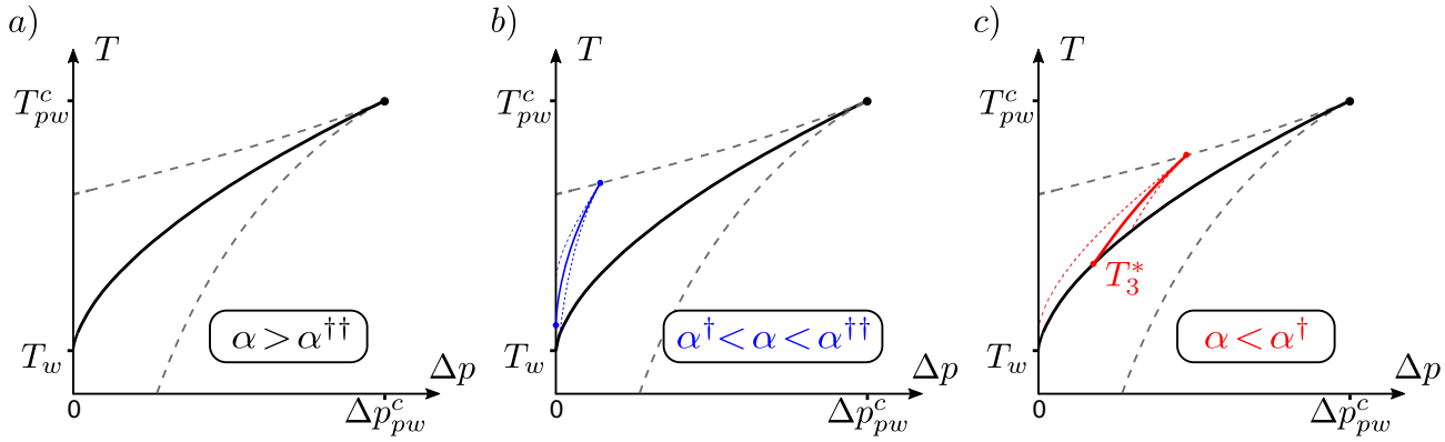
Fig. 11 Surface phase diagram for first-order wetting near an apex tip computed numerically using the binding potential (7): a) \alpha > \alpha^{\dagger\dagger} , for which no unbending line exists, b) \alpha^{\dagger} < \alpha < \alpha^{\dagger\dagger} , for which the unbending (blue) and pre-wetting (black) lines are separate, and c) \alpha < \alpha^{\dagger} , where the unbending (red) and pre-wetting (black) lines merge tangentially at T_3^* . The dashed lines represent the corresponding spinodals.
