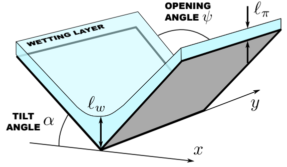
Fig. 2 Schematic illustration of an interfacial configuration in a shallow wedge showing the mid-point height \ell_w and planar wetting film thickness \ell_\pi . Translational invariance is assumed along the y -axis of the wedge.
