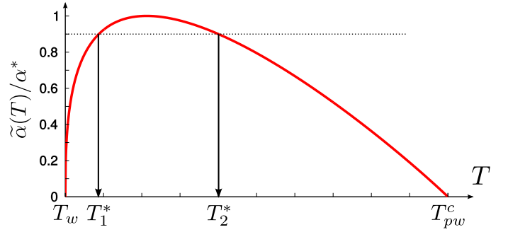
Fig. 7 The curve \tilde{\alpha}(T) computed numerically for the potential (7). For a given tilt angle \alpha < \alpha^* , the intersection of a horizontal line with this curve determines the temperatures T_1^* and T_2^* at which the pre-wetting and pre-filling lines merge.
