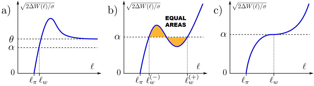
Fig. 3 Graphical construction for the equilibrium mid-point height \ell_w at different points of the phase diagram: a) For a first-order filling transition at bulk coexistence. The intersection of \sqrt{2\Delta W(\ell)}/\sigma with the horizontal line at height \alpha determines \ell_w . For \alpha < \theta , only one solution exists. For \theta = \alpha , corresponding to the filling transition phase boundary, microscopic and macroscopic adsorptions of liquid in the wedge coexist. b) At a point along the pre-filling line for which phases with different filling heights \ell_w^{(-)} and \ell_w^{(+)} coexist. The orange regions have equal areas. c) At a pre-filling critical point. An equal areas construction is no longer possible when the function \Delta W(\ell) has a point of inflection implying that the pre-filling point lies necessarily on the line of spinodals for the pre-wetting transition. These graphical constructions can also be interpreted as phase-portraits (\eta, \dot{\eta}) .
