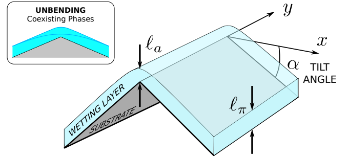
Fig. 8 Schematic illustration of an interfacial configuration near an apex showing the reduction of the local adsorption of liquid near the tip. Inset: Coexisting interfacial profiles at an unbending transition.
