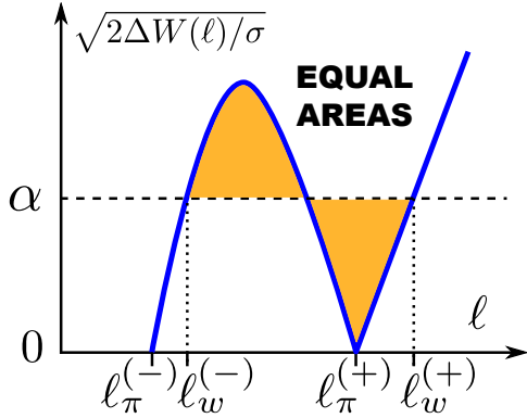
Fig. 6 Equal areas construction determining the merging of the pre-filling and pre-wetting lines (see text for details). This construction is equivalent to that determining the location of a first-order wetting transition within the Cahn theory of wetting for the case of zero surface enhancement 8,9 .
