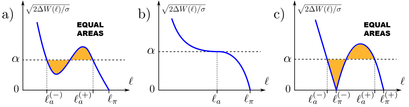
Fig. 9 Representative graphical constructions determining the surface phase diagram for fluid adsorption near an apex tip: a) equal areas construction for an unbending transition showing coexisting profiles with different thin ( \ell_a^{(-)} ) and thick ( \ell_a^{(+)} ) mid-point heights, b) an unbending critical point occurring off bulk liquid-gas coexistence, c) simultaneous occurrence of unbending and pre-wetting. Moving along the pre-wetting line, this latter construction is used in the determination of \bar{\alpha}(T) .
