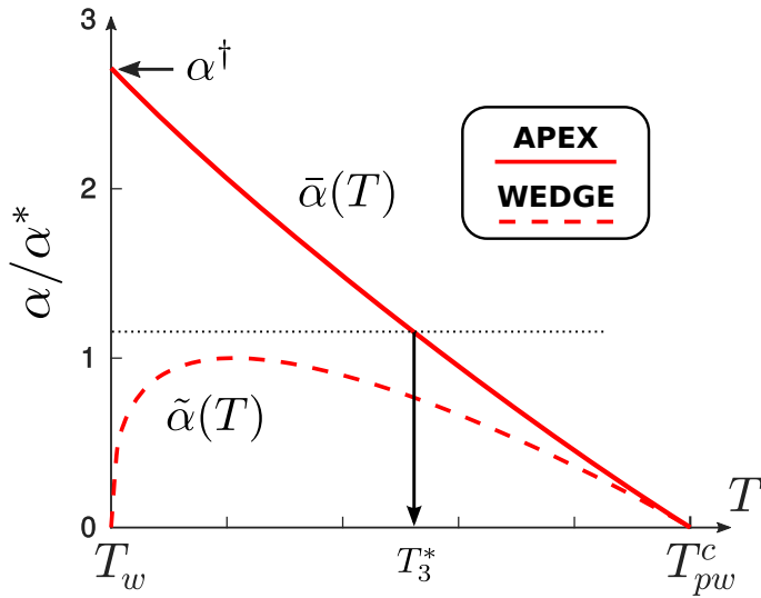
Fig. 10 The curve \bar{\alpha}(T) computed numerically for the potential (7). For a given tilt angle \alpha < \alpha^{\dagger} , the intersection of a horizontal line with this curve determines the temperatures T_3^* at which the pre-wetting and unbending lines merge. The curve \tilde{\alpha}(T) for a wedge is shown for comparison.
