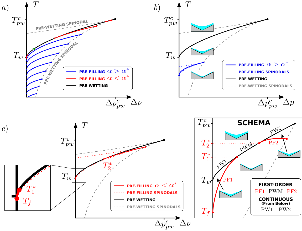
Fig. 4 Surface phase diagram for first-order wedge-filling transitions computed numerically using the binding potential (7): a) Pre-filling lines for different values of the tilting angle \alpha . Each of these lines finishes at a critical point that lies at the (lower) pre-wetting spinodal line. As \alpha decreases, the pre-filling line moves towards the pre-wetting line (in black). For \alpha > \alpha^* (blue lines), they do not touch the pre-wetting line. In the limiting case \alpha = \alpha^* , the pre-filling line touches the pre-wetting line tangentially at a single point, represented by the green circle. For \alpha < \alpha^* (red lines), the pre-filling lines consist of two parts that touch the pre-wetting line at two points, one at each side of the green point. b) For \alpha \approx 4.2\alpha^* , the surface phase diagram shows separate pre-filling and pre-wetting lines which do not intersect. The lower pre-filling spinodal follows closely the pre-filling line and merges with it at both ends, in sharp contrast with the lower pre-wetting spinodal, which only merges with the pre-wetting line at its critical point. Three schematic configurations of the interface at different points of the diagram are also shown. The phase diagram shows two transitions: First-order pre-filling (blue line) and continuous complete pre-wetting (black line). c) For \alpha \approx 0.80\alpha^* , the pre-filling lines (solid red) meet the pre-wetting line (solid black) tangentially at temperatures T_1^* and T_2^* . Note that the two parts of the pre-filling lines have common upper and lower spinodal lines (dashed red). The splitting of the pre-filling and pre-wetting line is shown schematically. There is no metastable continuation of the pre-filling line that joins the two points at T_1^* and T_2^*
