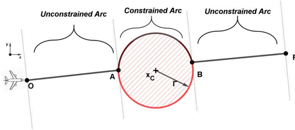
Figure 4.1: Schematic configuration of aircraft and fixed obstacle.
