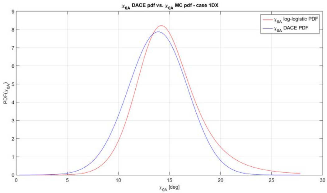
Figure 5.14: DACE and MC \chi_{0A} PDFs for 10^7 samples - case 1DX.
