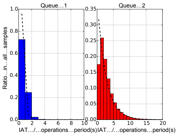
(b) IAT distributions in Scenario 2 under a random strategy, fitted as geometric distributions.
