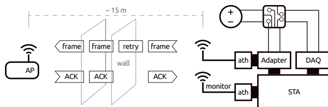
Figure 6: Experimental setup.
